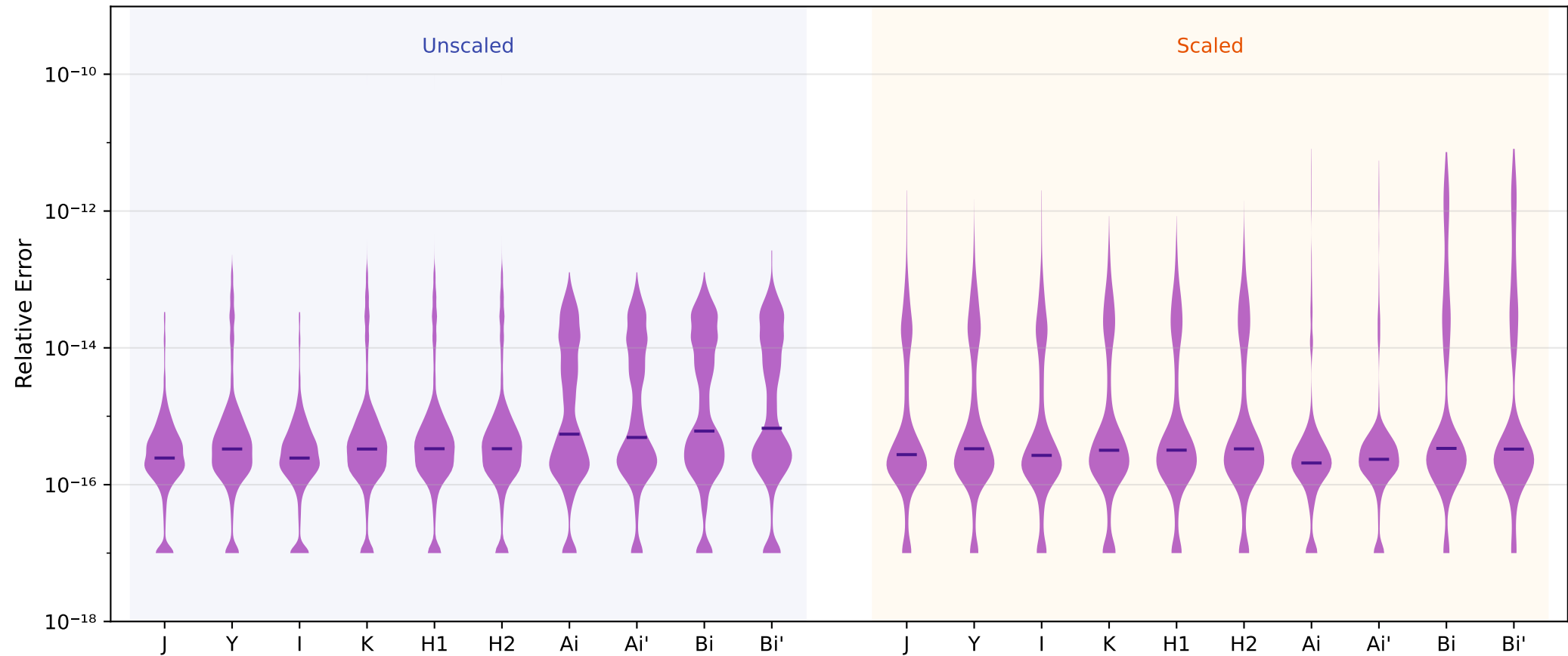
Implementation Fidelity — complex-bessel (Rust) vs AMOS/TOMS 644 (Fortran), \nu \geq 0
