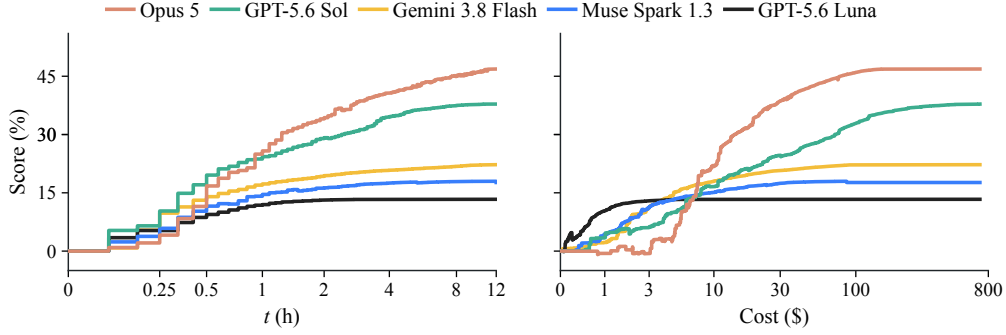
Figure 5: Compression increase is almost saturated after at most 2 h and $30 but continues to rise for GPT-5.6 Sol and Opus 5.
