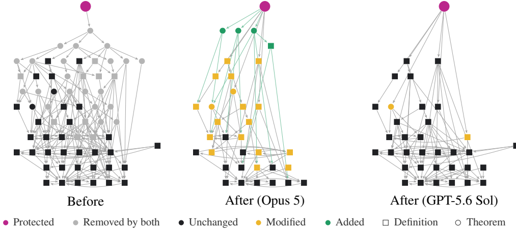
Figure 8: Dependency graphs for a repository before and after compression show that Opus 5 modifies and inserts declarations extensively, while GPT-5.6 Sol focuses on removing declarations.
