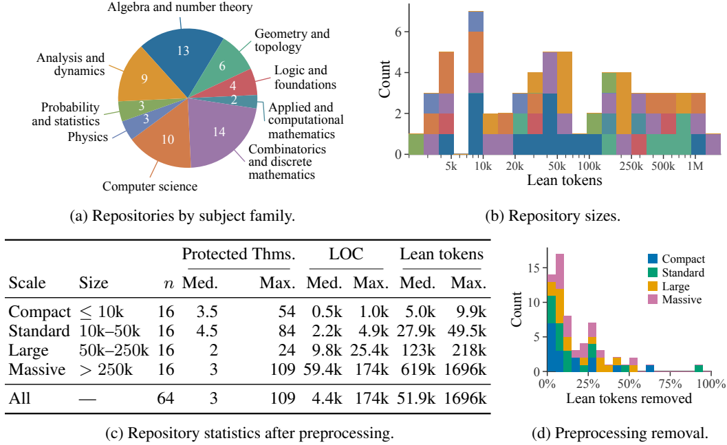
Figure 3: Composition and preprocessing of LEANLEAN. The 64 repositories cover diverse mathematical topics (a) and are balanced across repository sizes (b). The four size groups span a wide range of protected theorem counts, lines of code (LOC), and Lean tokens after preprocessing (c). Preprocessing removes a median of 10.7% unused Lean tokens across all four size groups (d).
