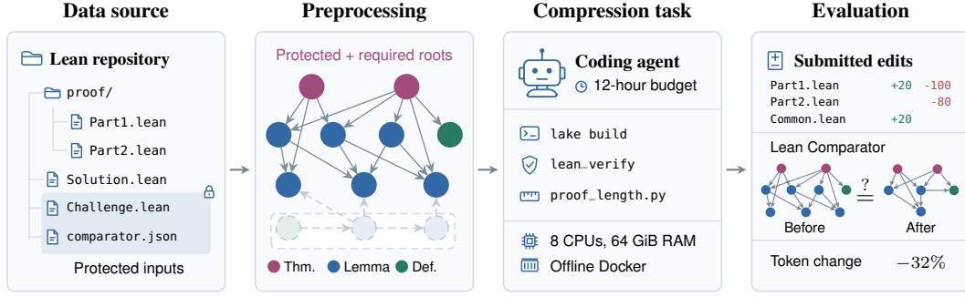
Figure 1: We construct LEANLEAN by collecting 64 Lean repositories from the Palomar Registry and removing declarations outside the dependency closure of the protected results and other required roots. An agent then has 12 hours to reduce the remaining Lean token count, with access to build, verification, and measurement tools. We rebuild the submitted repository and use the Lean Comparator to check that the protected results still hold under the permitted axioms.
