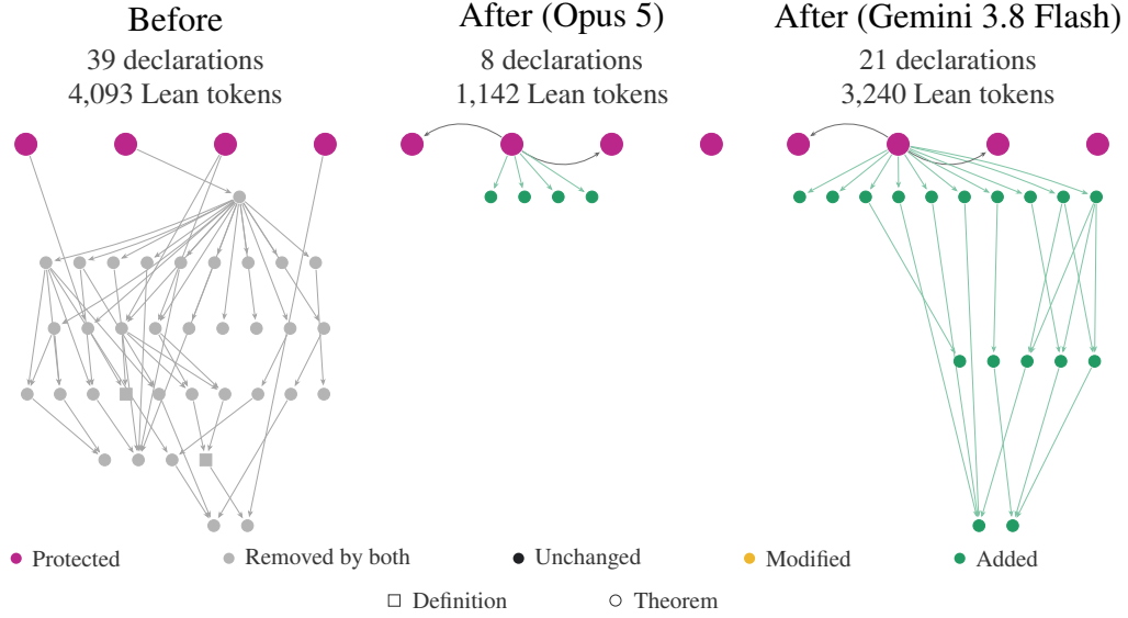
Figure 18: Declaration dependency graphs for the Morphic Numbers example before compression and after compression by Opus 5 and Gemini 3.8 Flash.
