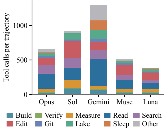
Figure 9: Tool calls per trajectory by model.
