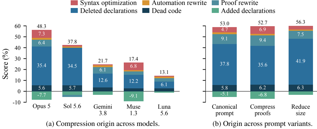
Figure 7: Most compression gains originate from deleting declarations that the proofs previously depended on (a), often enabled by extensive proof rewrites. Opus 5’s strategies do not change depending on the instruction (b).
