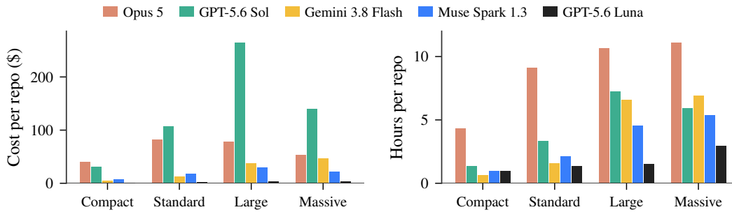
Figure 16: Mean cost per repository in USD (left) and mean duration per repository in hours (right) by repository scale for each evaluated model.
