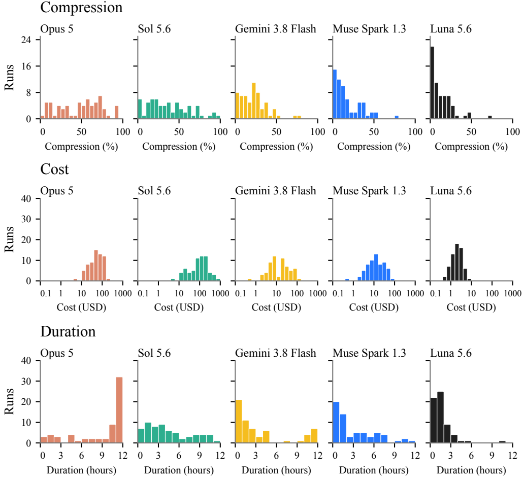
Figure 15: Histograms of compression scores (top), task cost (middle), and task duration (bottom) per model. Cost is shown on a logarithmic scale.
