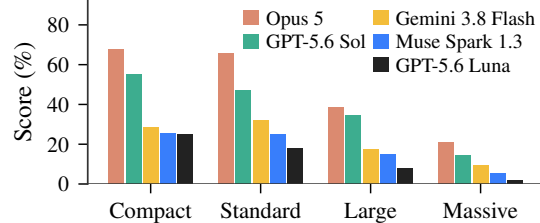
Figure 6: Compression drops with repository scale.
