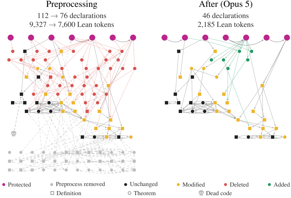
Figure 17: Dependency graphs for Tucker’s lemma before preprocessing (left) and after Opus 5 compression (right).
