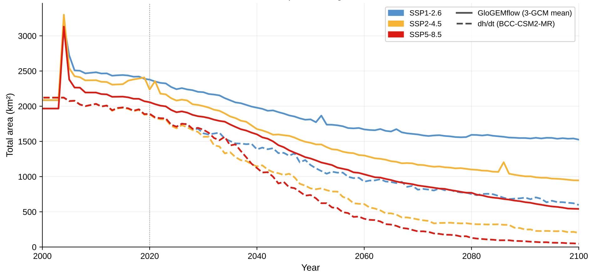
Central Europe — total glacier area
