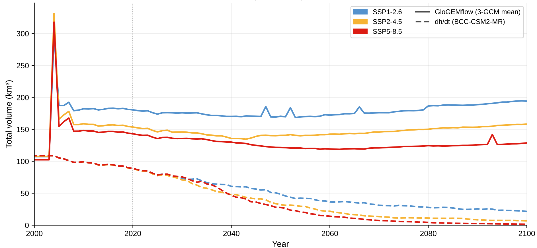
Central Europe — total glacier volume
