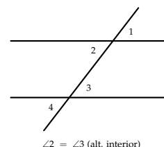
\angle 2 = \angle 3 (alt. interior)
