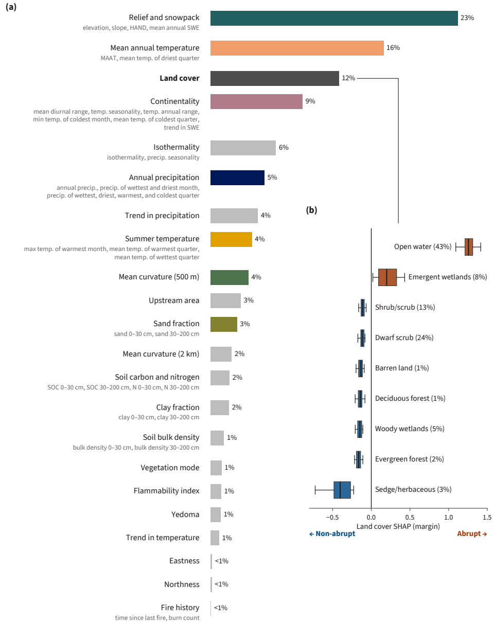
Figure 6. Grouped SHAP importance of environmental variables. (a) Environmental variables are organized into 22 feature families based on their correlation structure, ranked by their SHAP importance on held-out observations under spatial cross-validation, with percentages showing each family's share of total importance. Family importance is the mean absolute value of the summed SHAP values of the family's members. Member variables are listed in grey beneath each multi-member family. Colored bars denote the seven families that are shown individually on the map in Figure 8. (b) Summed SHAP values for the land cover family, grouped by land cover class, only showing classes with at least 100 observations. Percentages show each class's share of observations. Boxes span the interquartile range, whiskers span the 5th to 95th percentiles, and classes are ordered by median SHAP value.
