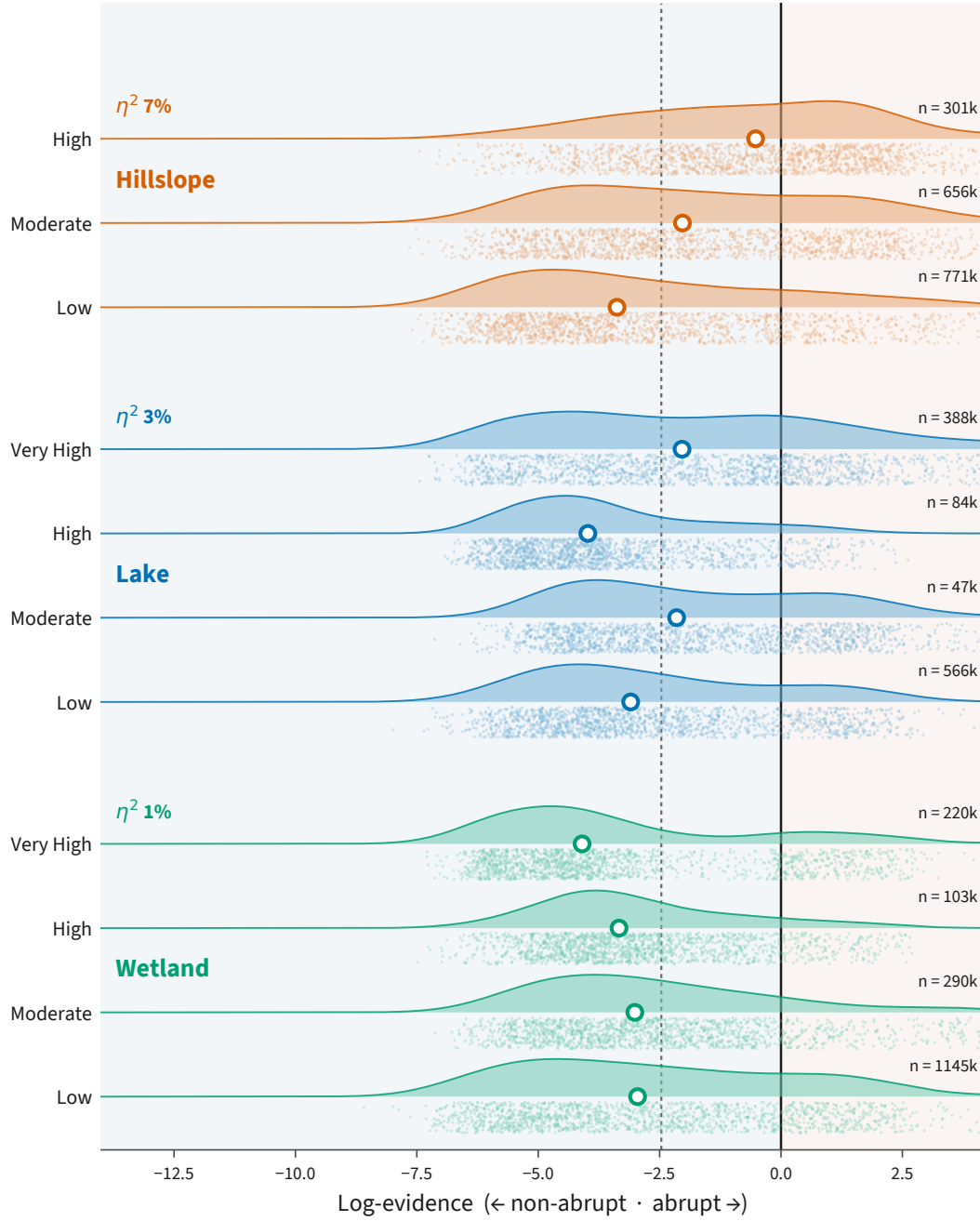
Figure 10. Thaw mode across thermokarst landform classes. Distributions of in-AoA log-evidence by thermokarst type and occurrence potential from Olefeldt et al. (2016). Curves show density, circles mark medians, solid and dashed vertical lines mark neutral log-evidence and the statewide median, respectively. Points sub-sample grid cells. Annotated \eta^2 values give the variance in log-evidence explained by occurrence potential within each thermokarst type, and n gives the number of in-AoA grid cells. “None” classes are excluded.
