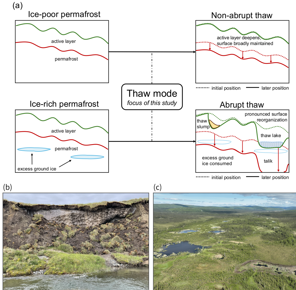
Figure 1. Conceptual illustration of permafrost thaw mode. Idealized cross-sections (a), not drawn to scale, contrasting the two thaw modes and the ground-ice characteristics of each. Ice-poor permafrost (top left) leads to non-abrupt thaw (top right), where the active layer may deepen but the surface is broadly maintained, allowing gradual subsidence at most. Ice-rich permafrost (bottom left) undergoes abrupt thaw (bottom right) when excess ground ice is removed, leading to pronounced surface reorganization. Field photographs show two examples of abrupt thaw landforms: a thaw slump along an eroding riverbank in Alaska’s North Slope (b), photographed by Irina Overeem, and a drone image of a thermokarst wetland in Goldstream Valley (c), photographed by Kevin Rozmiarek.
