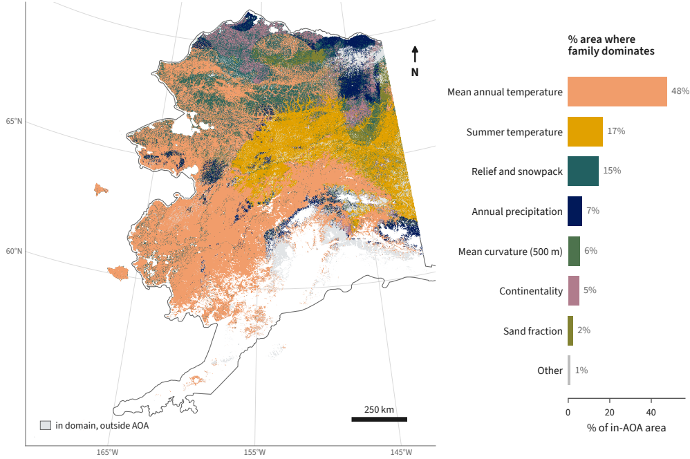
Figure 8. Spatial distribution of dominant indicators. Each in-AoA grid cell is colored by the family with the largest-magnitude net SHAP contribution from the final model. Bars show the percentage of in-AoA grid cells dominated by each group. Grey shading marks terrain within the permafrost domain but outside AoA.
