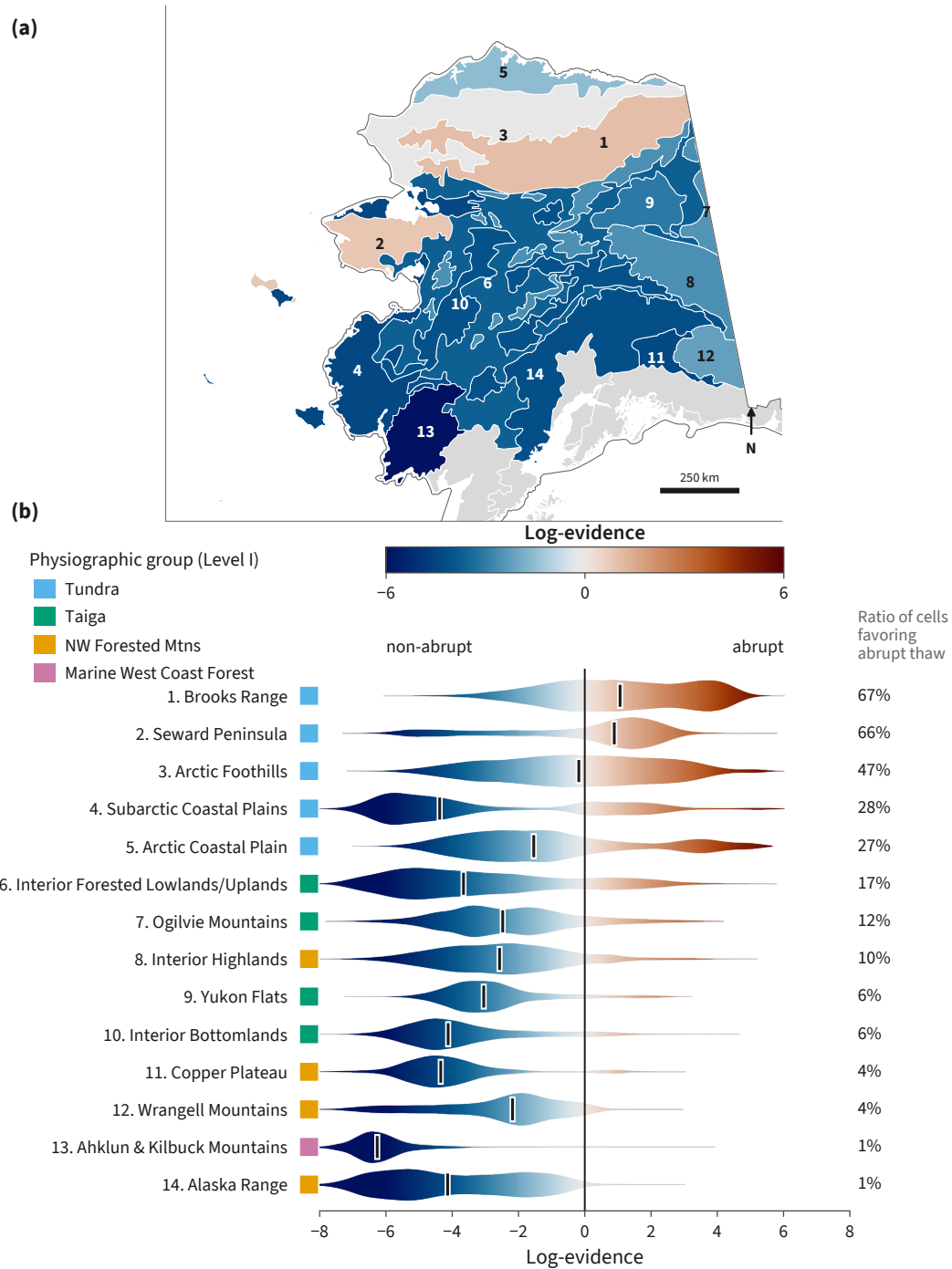
Figure 9. Regional variation in thaw mode. (a) Median log-evidence by Level III ecoregion. (b) Distributions of in-AoA log-evidence within each ecoregion, ranked by the percentage favoring abrupt thaw. Ticks mark medians and colored squares denote Level I physiographic groups. Only regions with at least 50% permafrost coverage are shown, and all retained regions have at least 80% AoA coverage.
