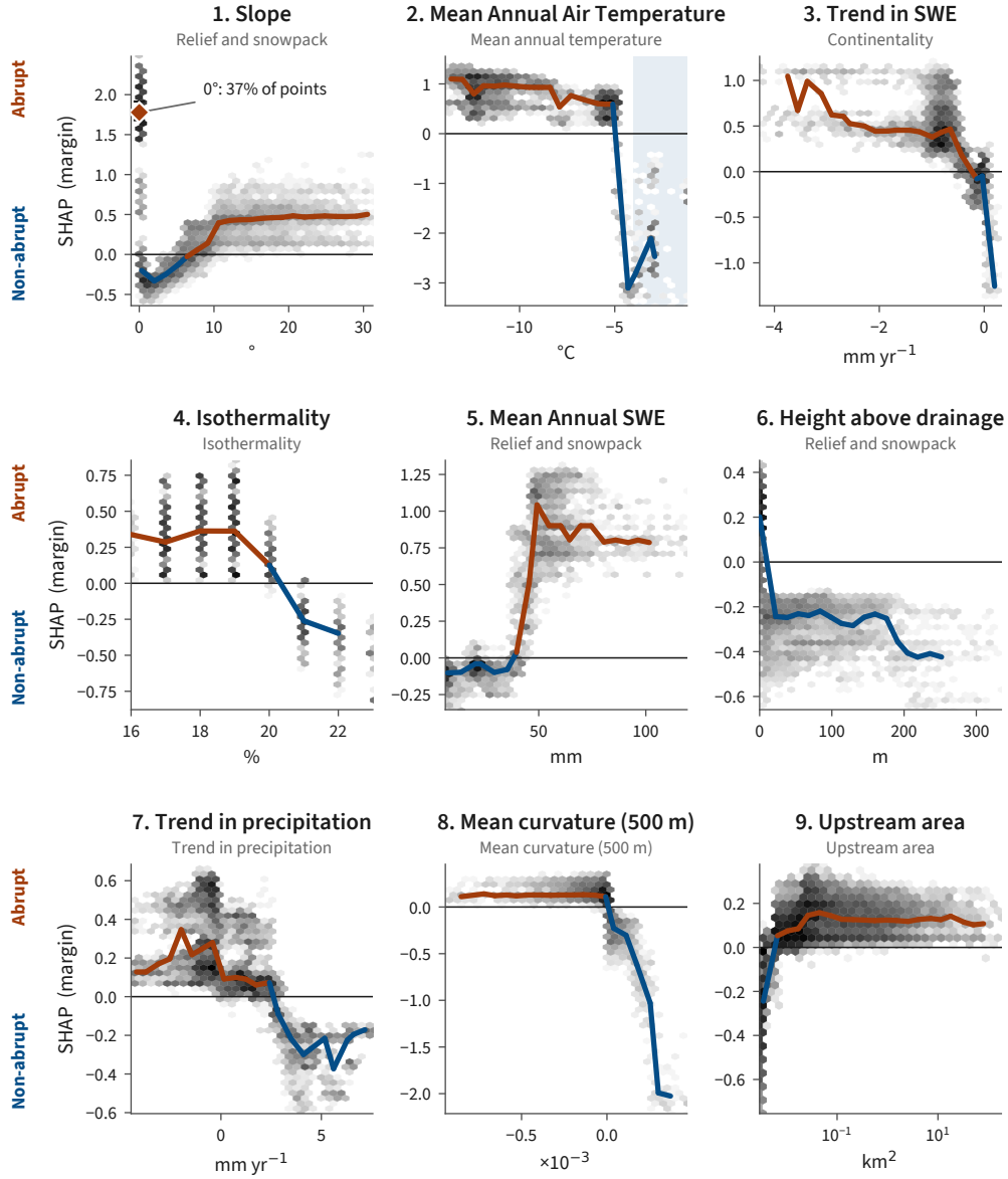
Figure 7. Individual SHAP response plots for leading indicators. SHAP values for the nine most influential continuous variables on held-out observations, ranked by mean absolute importance, ordered from top-left to bottom-right. Subtitles indicate which family each panel belongs to. Grey shading shows observation density, while binned median responses show where each variable favors abrupt (orange, positive y) or non-abrupt (blue, negative y) thaw. Note that vertical and horizontal scales vary among panels.
