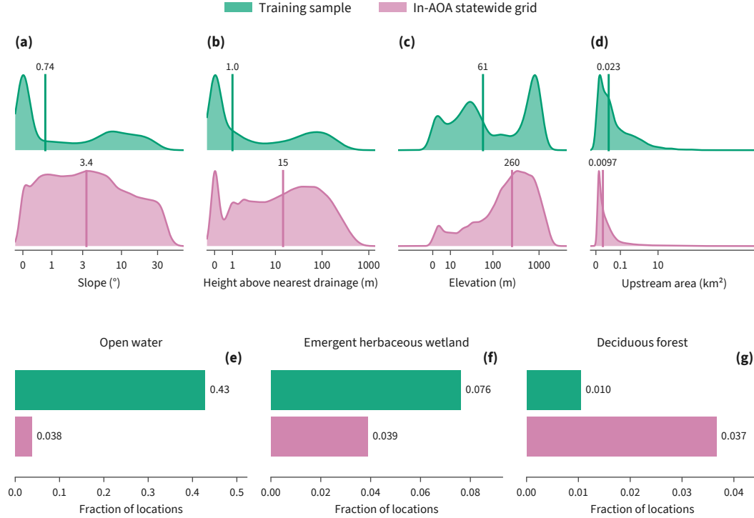
Figure 4. Representativeness of the training sample. Distributions of selected environmental features in the training sample (green) and across the statewide grid within the area-of-applicability (pink). Continuous variables shown are slope (a), height above nearest drainage (b), elevation (c), and upstream drainage area (d). Densities are independently normalized, with vertical lines and annotations denoting the median of each respective distribution. Note that the horizontal axes use an inverse-hyperbolic-sine transform, approximately linear near zero and logarithmic at large values. Categorical variables shown are the land cover fraction of open water (e), emergent herbaceous wetlands (f), and deciduous forest (g).
