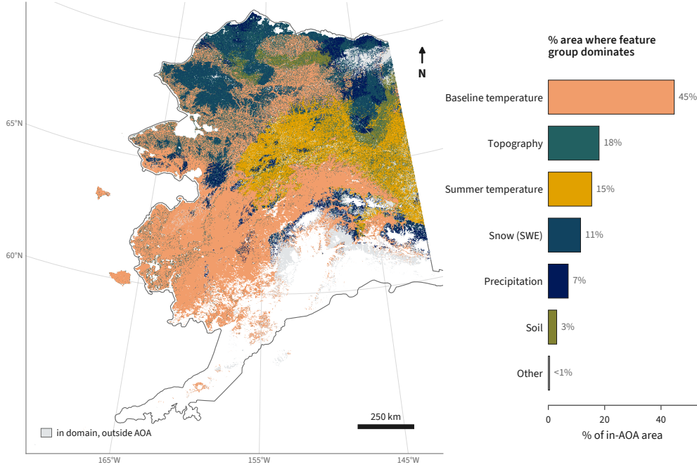
Figure 9. Spatial distribution of dominant indicators. Each in-AoA grid cell is colored by the thematic domain with the largest-magnitude net SHAP contribution from the final model. Bars show the percentage of in-AoA area dominated by each group. Grey shading marks terrain within the permafrost domain but outside AoA.
