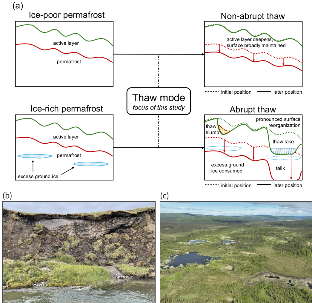
Figure 1. Conceptual illustration of permafrost thaw mode. Idealized cross-sections (a), not drawn to scale, contrasting the two thaw modes and the ground-ice characteristics of each. Ice-poor permafrost (top left) leads to non-abrupt thaw (top right), where the active layer may deepen but the surface is broadly maintained, allowing gradual subsidence at most. Ice-rich permafrost (bottom left) undergoes abrupt thaw (bottom right) when excess ground ice is removed, leading to pronounced surface reorganization. Field photographs show two examples of abrupt thaw landforms: a thaw slump along an eroding riverbank in Alaska's North Slope (b), photographed by Irina Overeem, and a drone image of a thermokarst wetland in Goldstream Valley (c), photographed by Kevin Rozmiarek.
