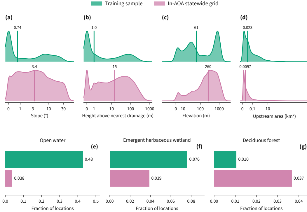
Figure 4. Representativeness of the training sample. Distributions of selected environmental features in the training sample (green) and across the statewide grid within the area-of-applicability (pink). Continuous variables shown are slope (a), height above nearest drainage (b), elevation (c), and upstream drainage area (d). Densities are independently normalized, with vertical lines and annotations denoting the median of each respective distribution. Note that the horizontal axes use an inverse-hyperbolic-sine transform, approximately linear near zero and logarithmic at large values. Categorical variables shown are the land cover fraction of open water (e), emergent herbaceous wetlands (f), and deciduous forest (g).
