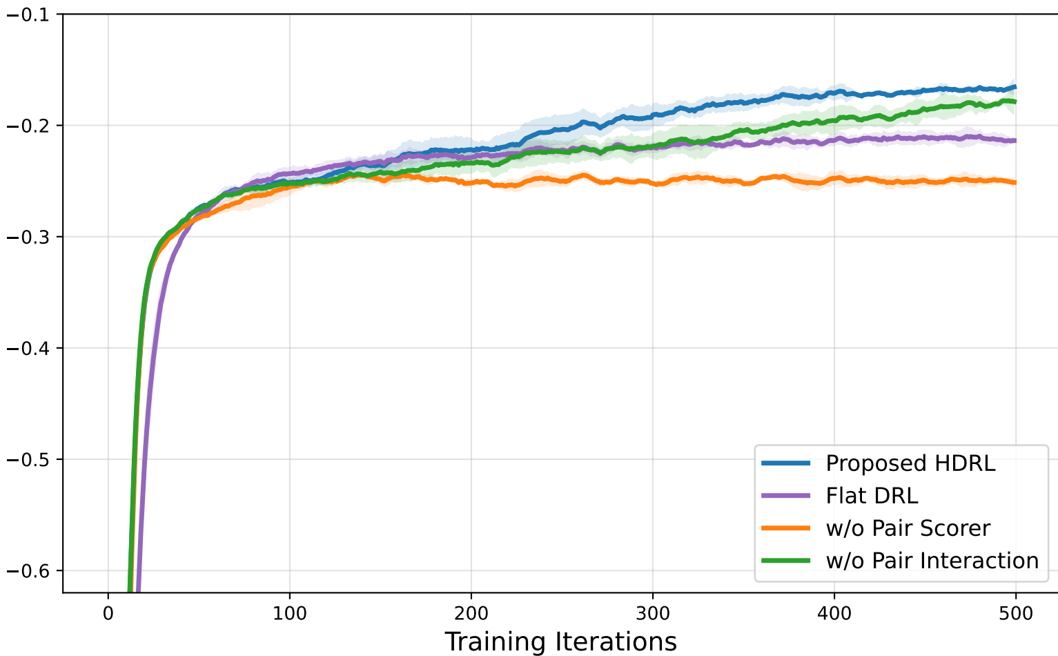
Average Low-Level Reward
