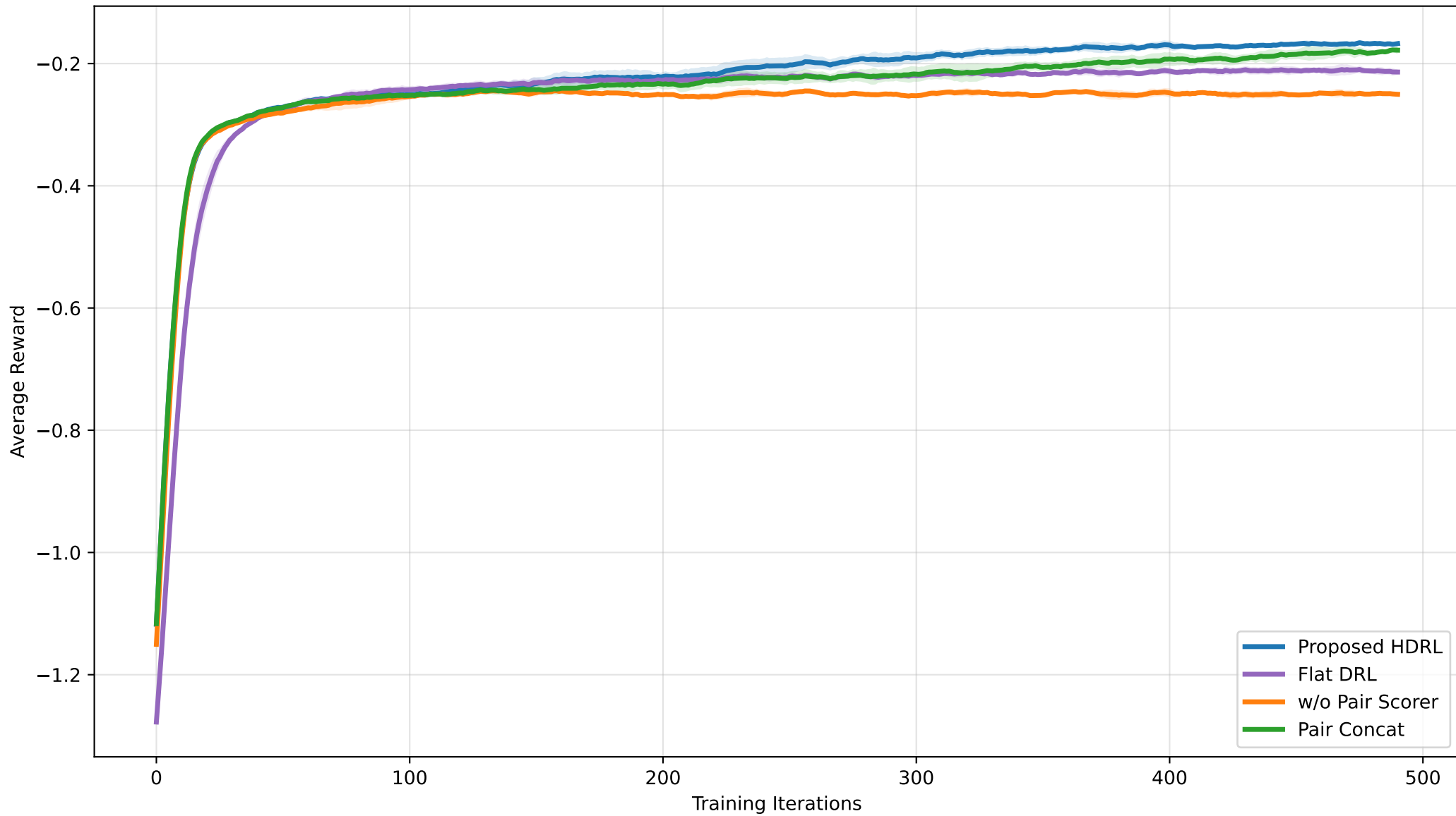
Convergence Comparison of DRL-Based Methods
