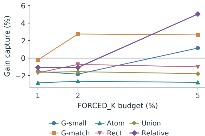
(a) COCO: all six models
