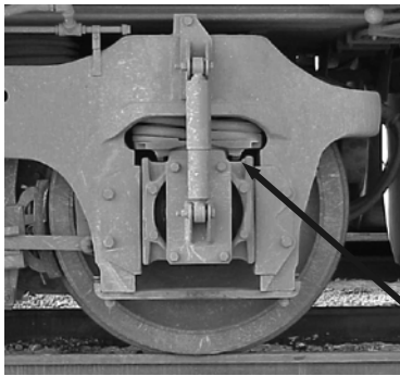
Locomotive Bearing
