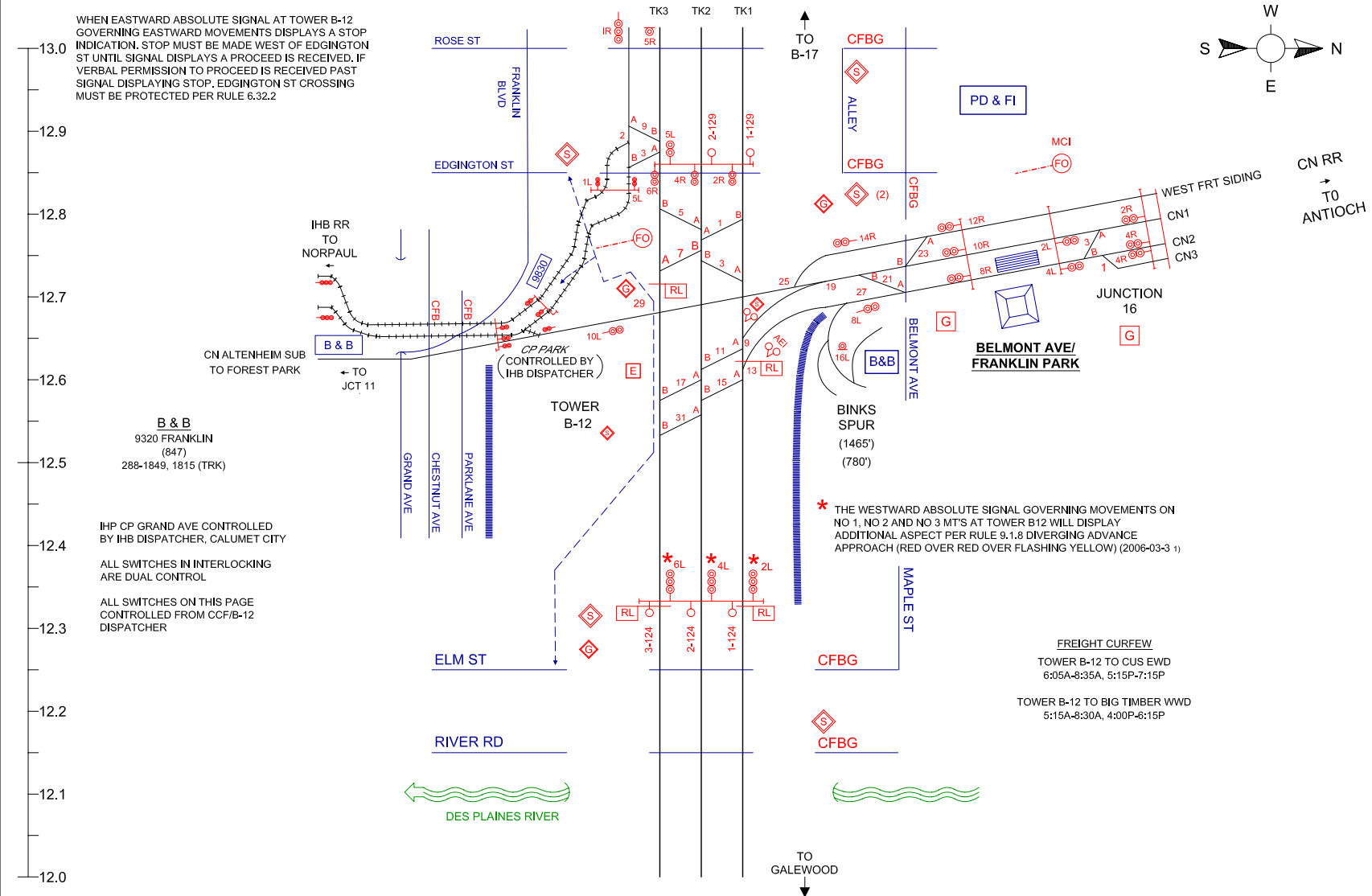
DETAIL VIEW OF TOWER B-12 INTERLOCKING
