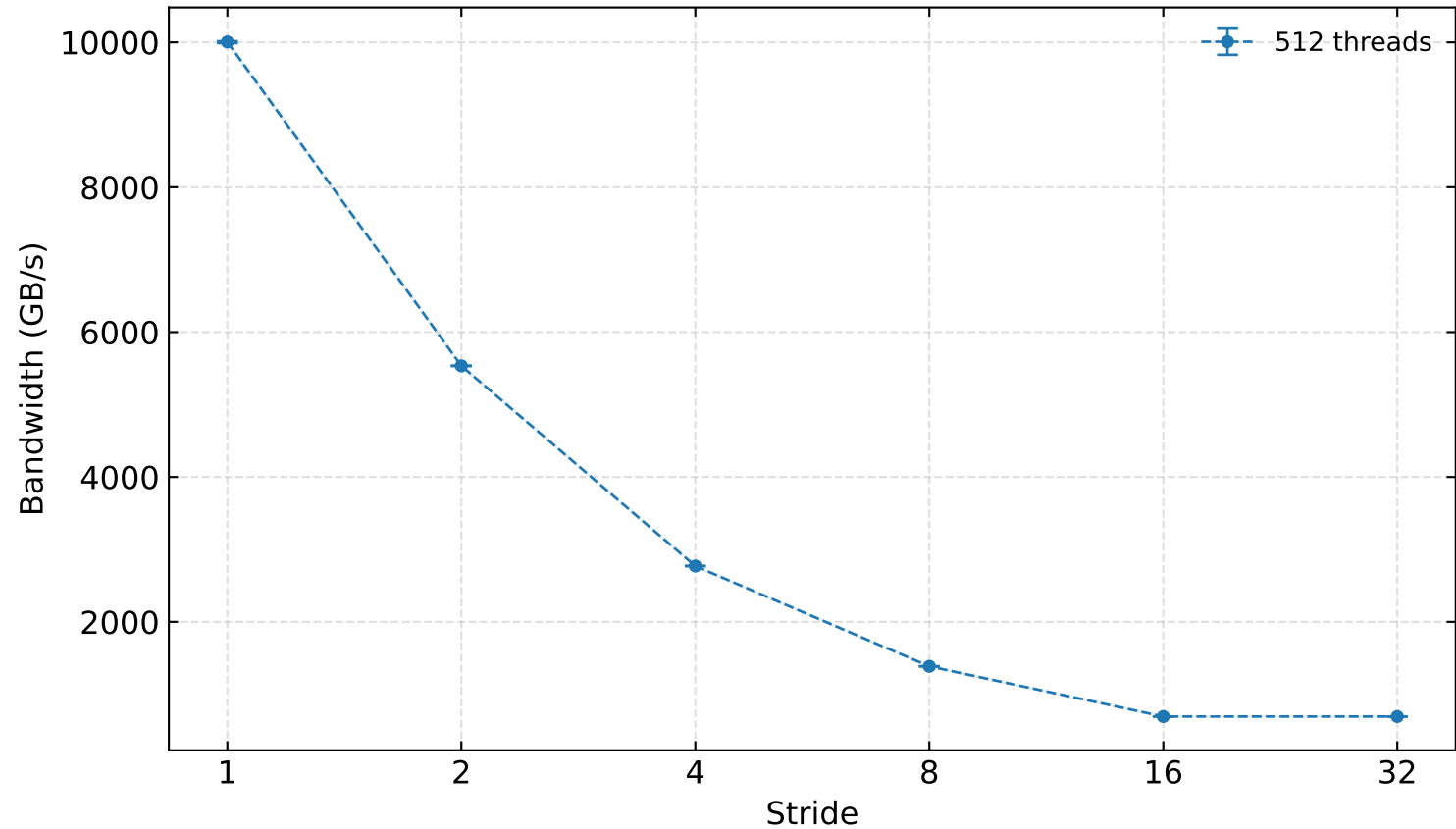
Shared Memory to Register Bandwidth (Single SM, 8 KiB read)
