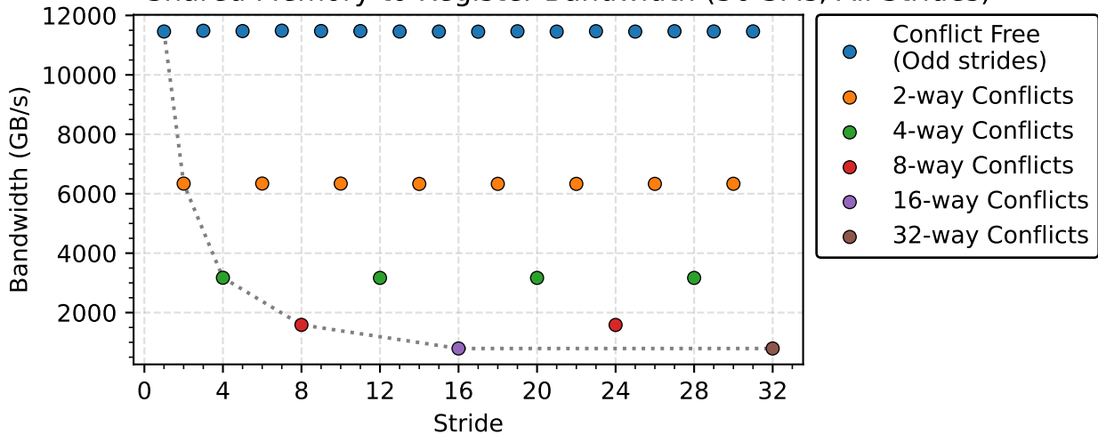
Shared Memory to Register Bandwidth (36 SMs, All Strides)
