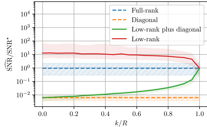
RBF RFFs
