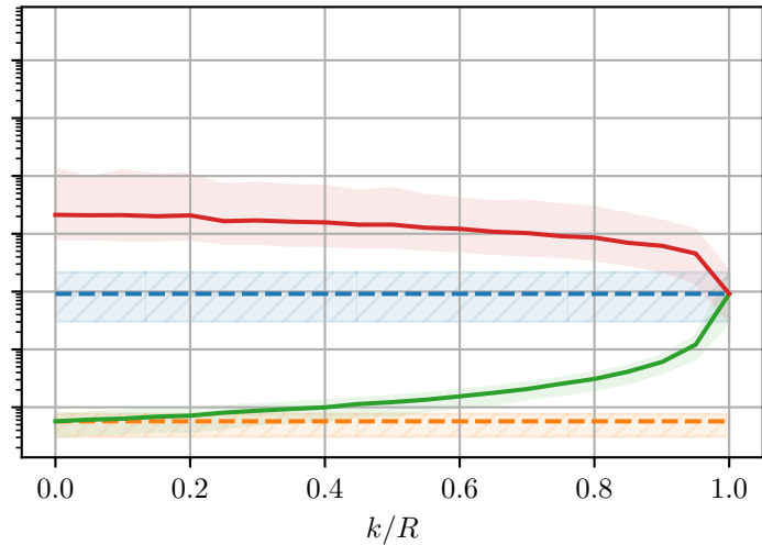
Matern RFFs
