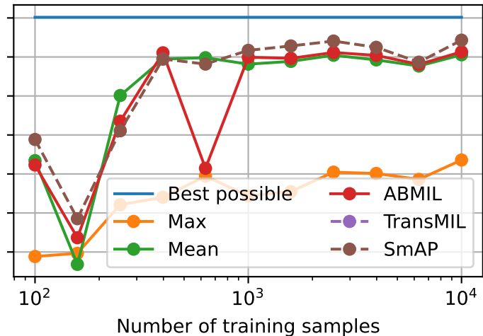
Prediction-aggregation approach
