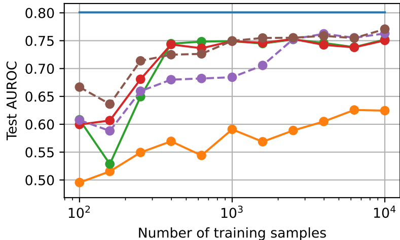
Embedding-aggregation approach
