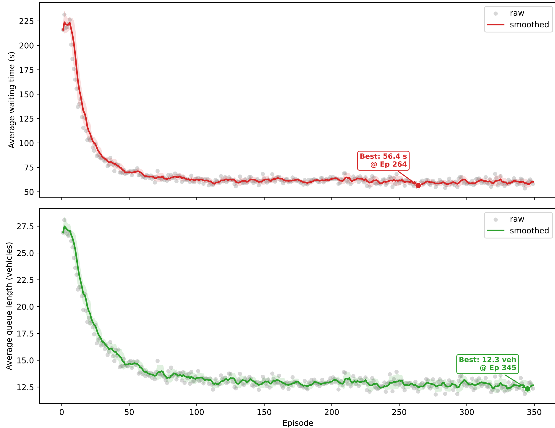
Queue reward dynamic LR training curve, run 3
