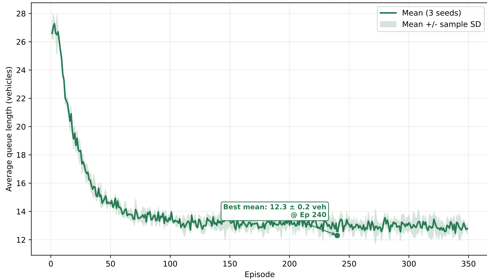
S02: three-seed queue-length learning curve
