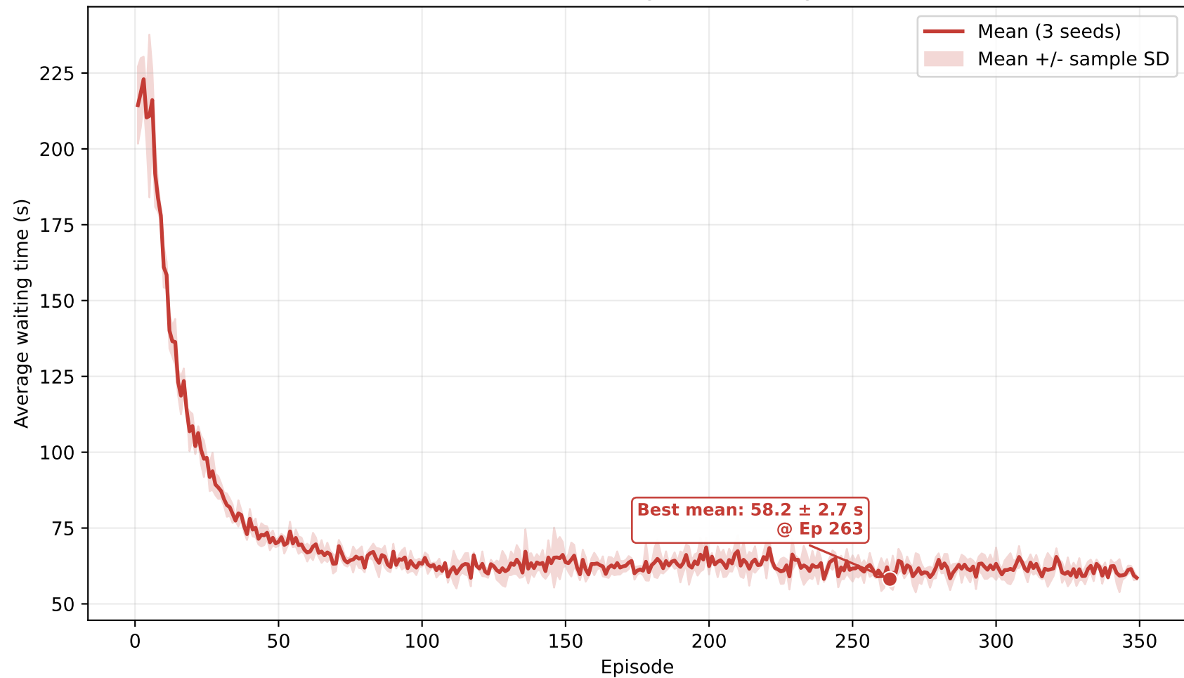
S02: three-seed waiting-time learning curve
