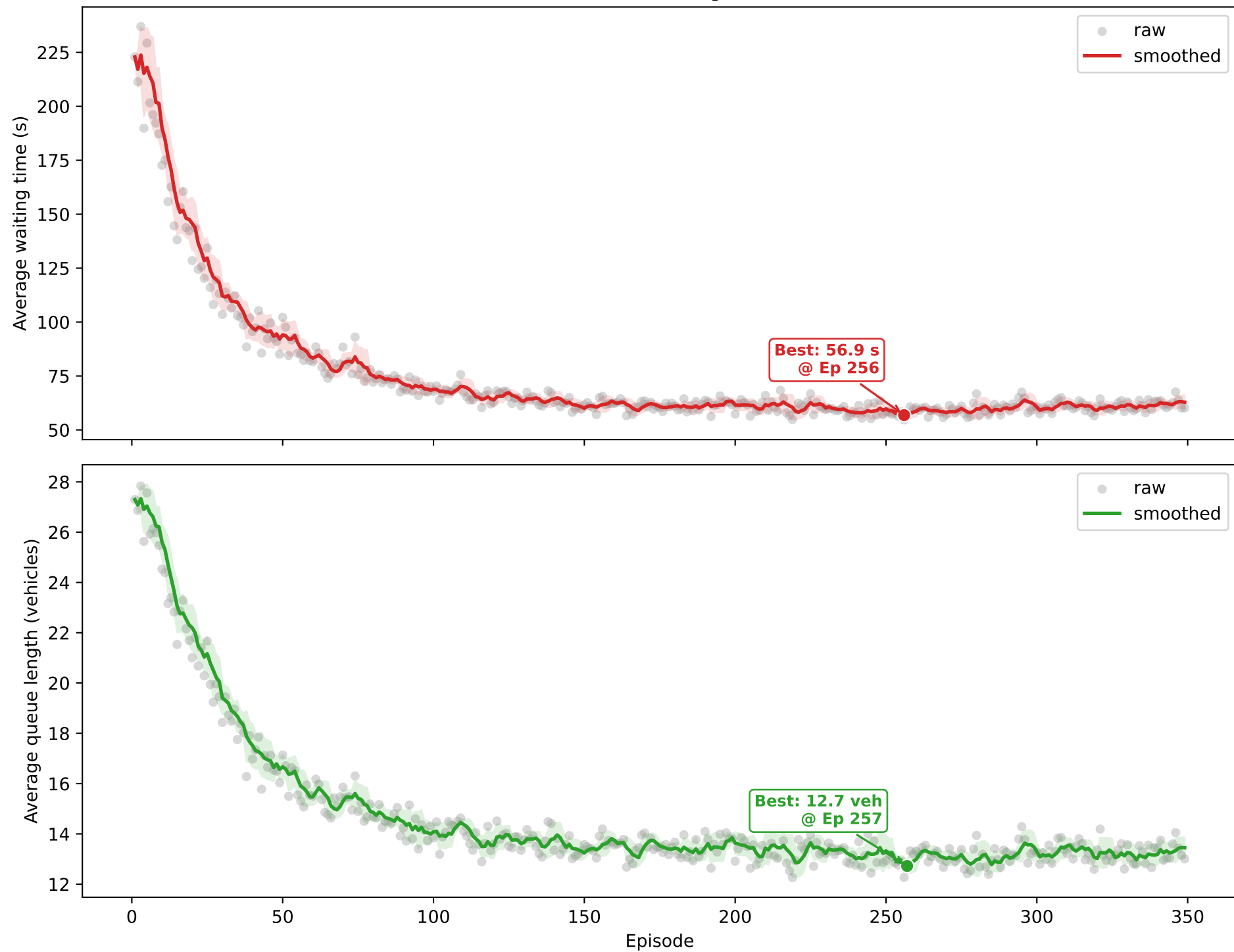
Potential reward training curve, run 3
