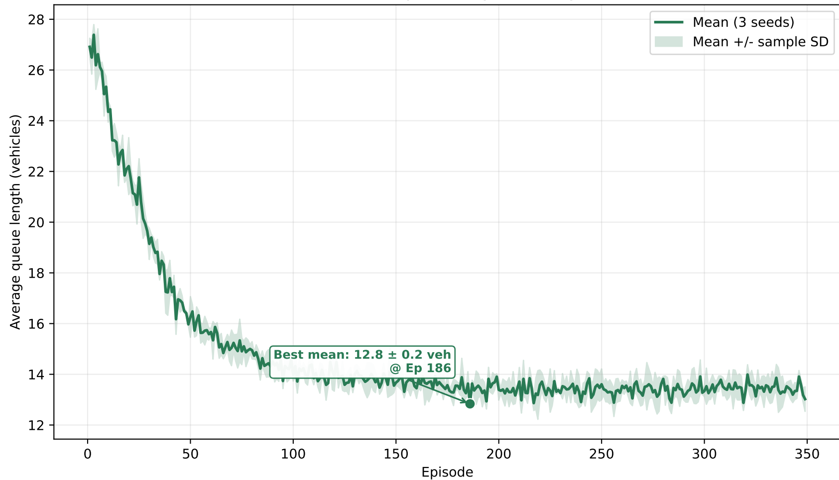
S03: three-seed queue-length learning curve
