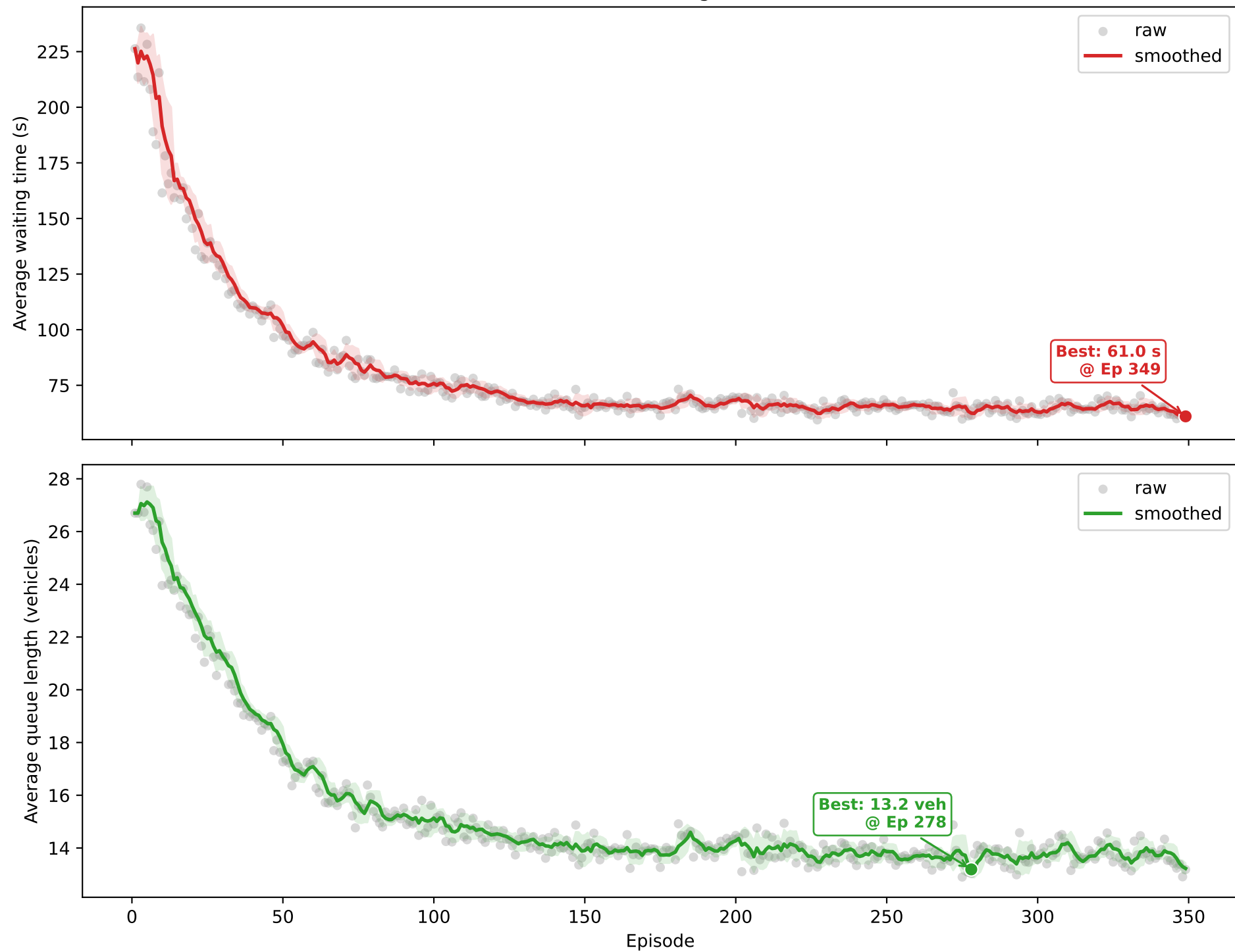
Queue reward training curve, run 2
