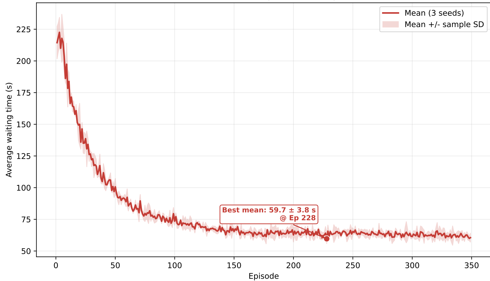
S01: three-seed waiting-time learning curve
