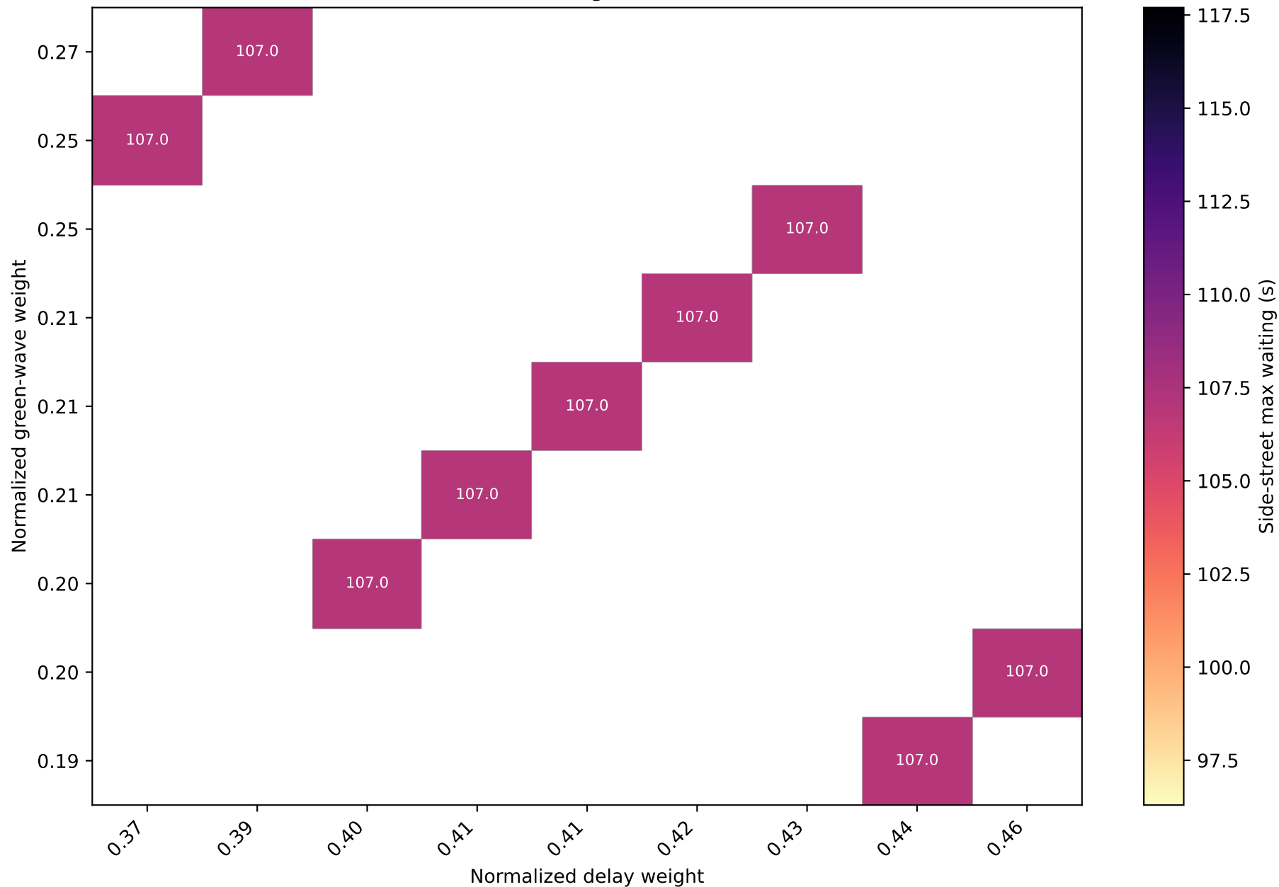
Run 1: Side-street Max Waiting across Tunable Preferences
