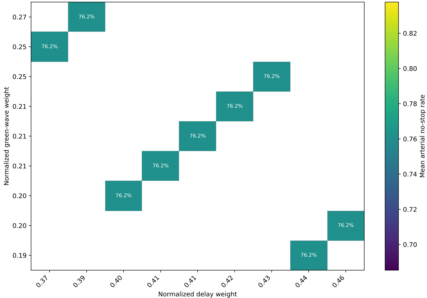
Run 2: No-stop Rate across Tunable Preferences
