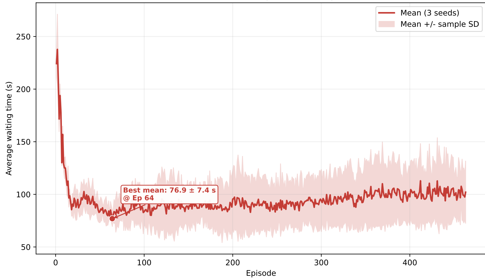
M06: three-seed waiting-time learning curve
