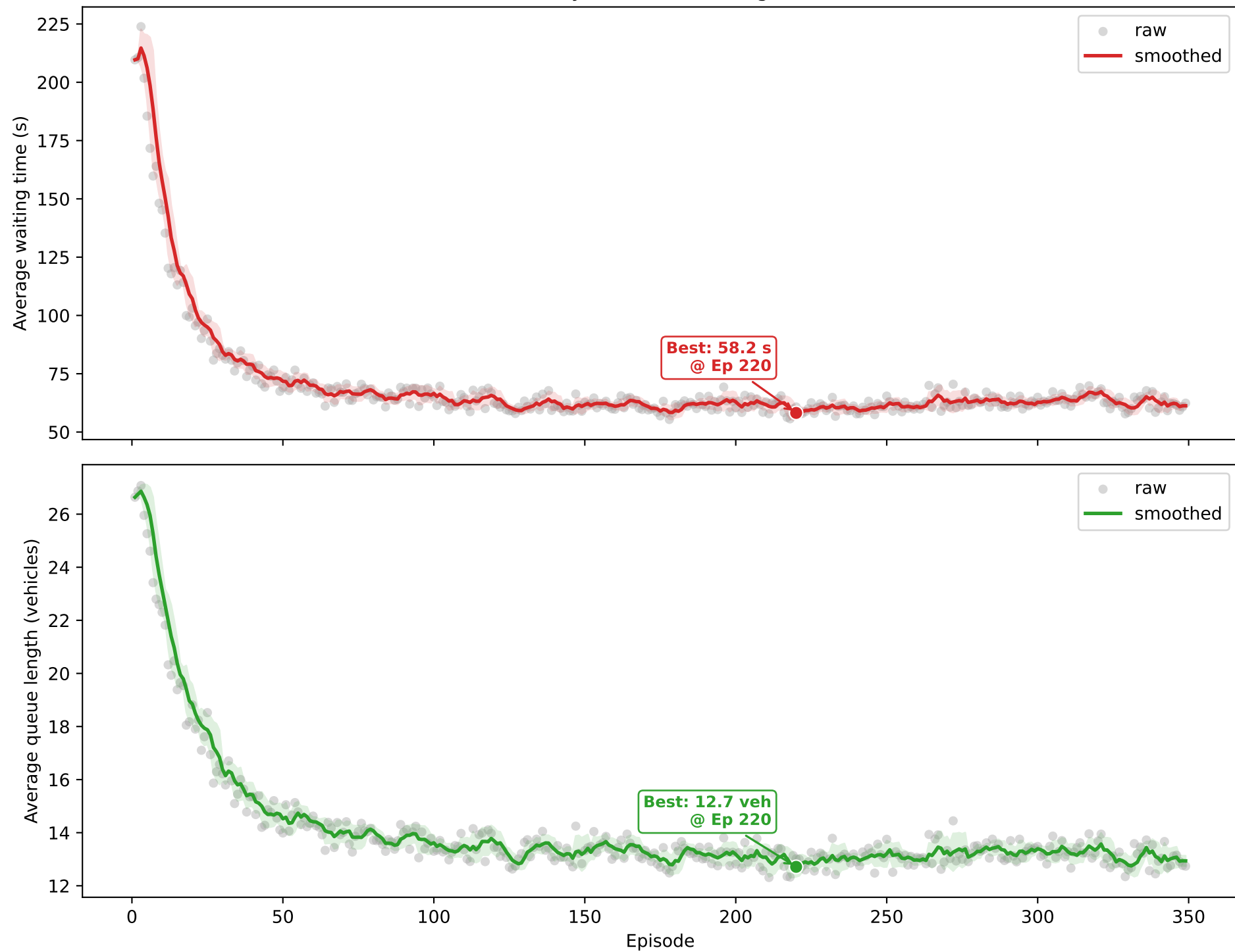
PBRS reward dynamic LR training curve, run 2
