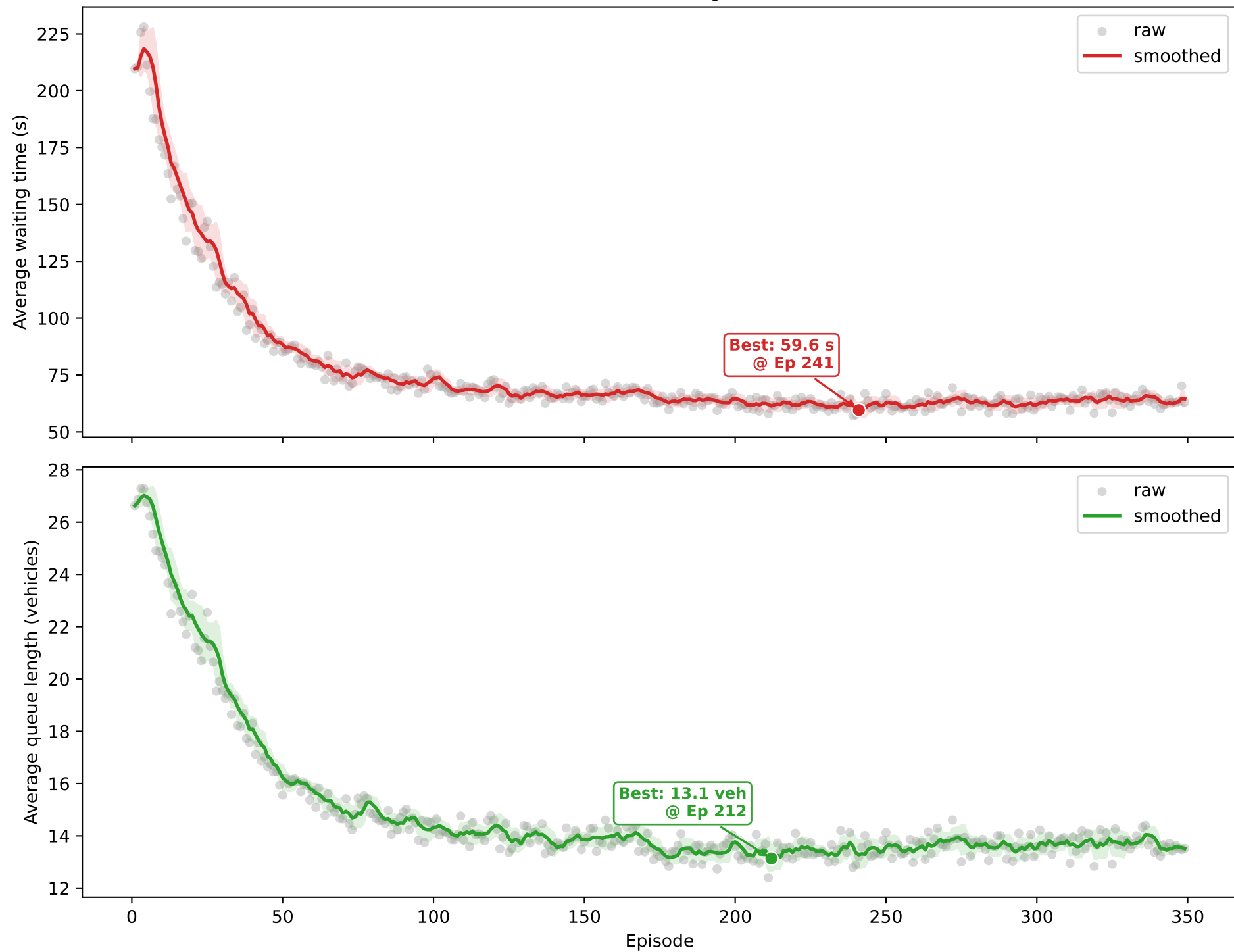
Potential reward training curve, run 2
