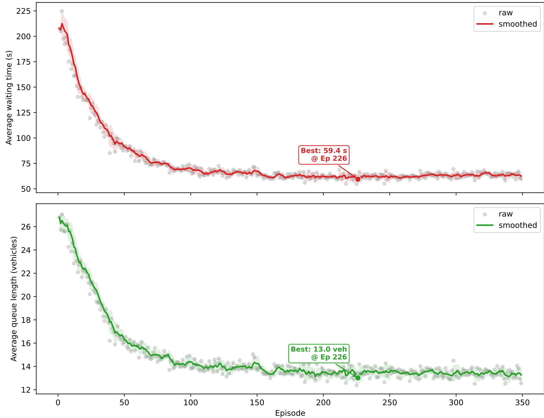
Potential reward training curve, run 1
