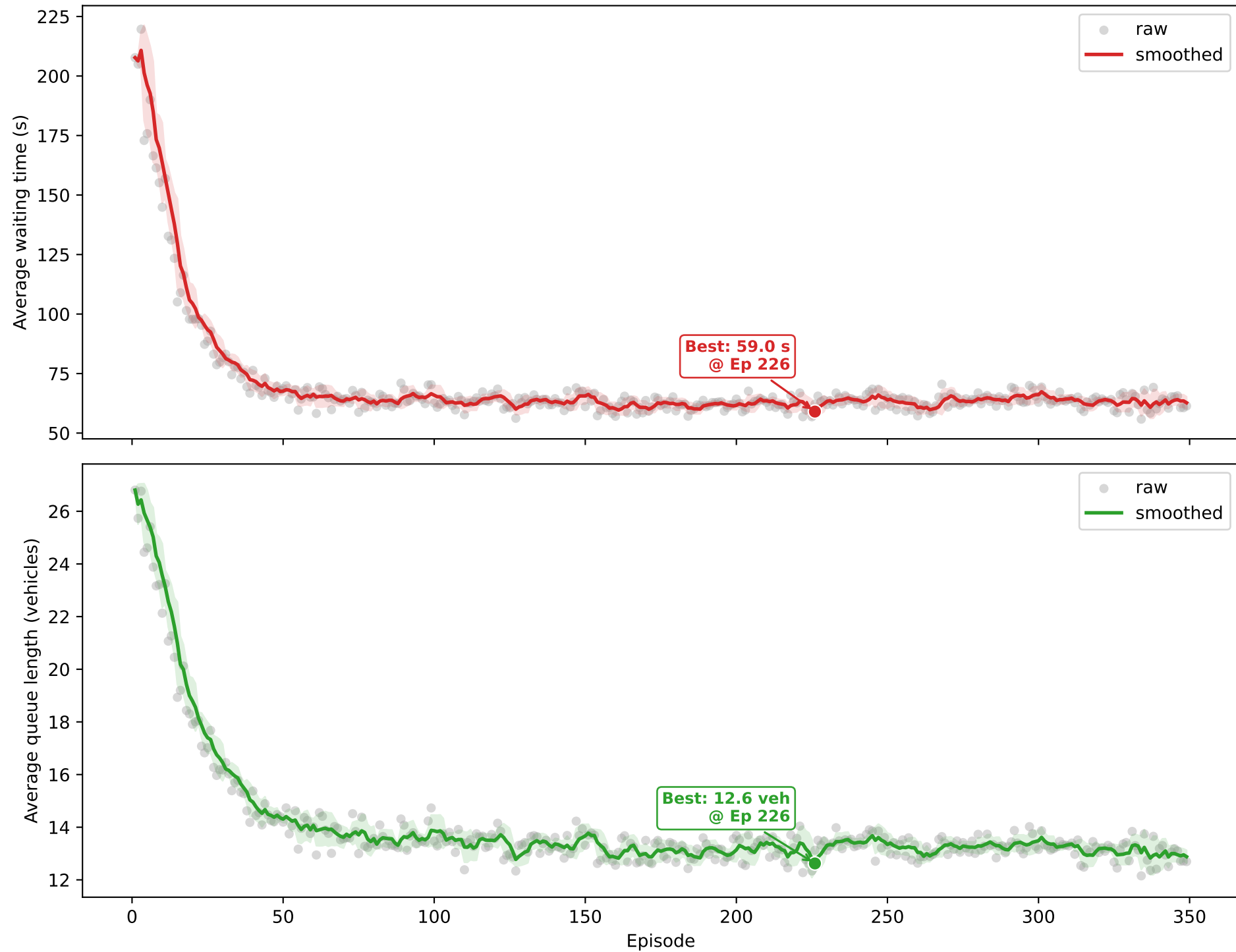
PBRS reward dynamic LR training curve, run 1
