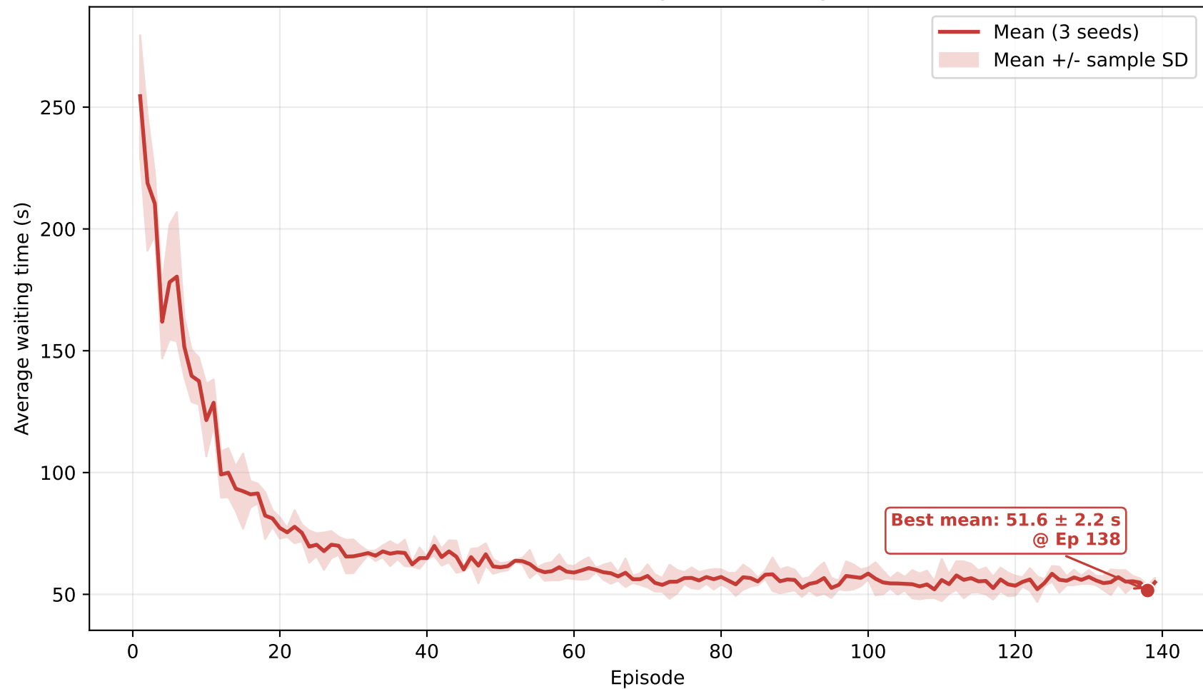
M04: three-seed waiting-time learning curve
