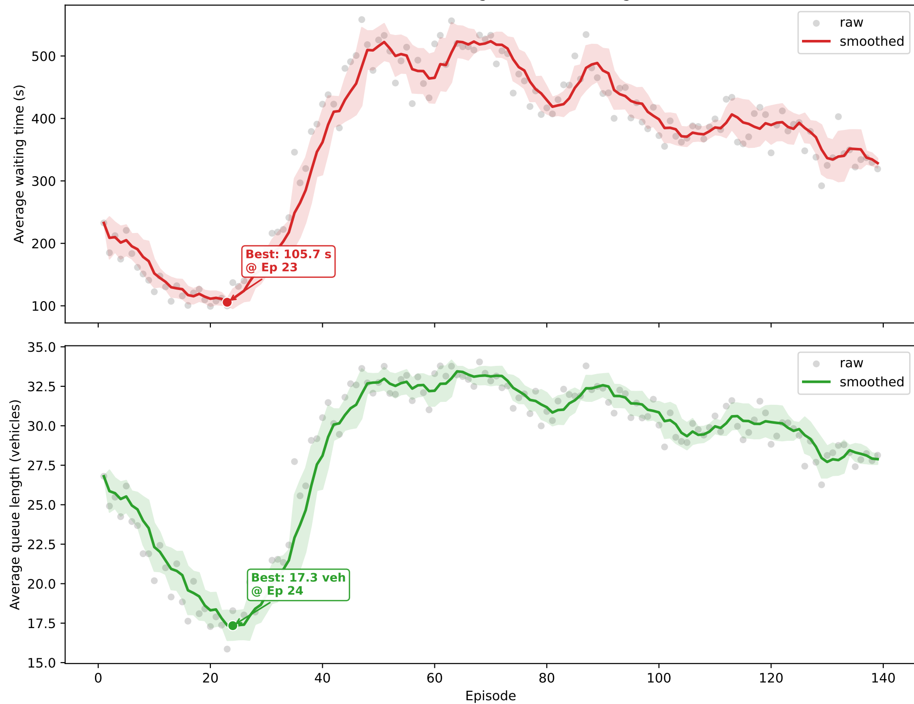
MARL PBRS communication green-wave waiting time, run 2
