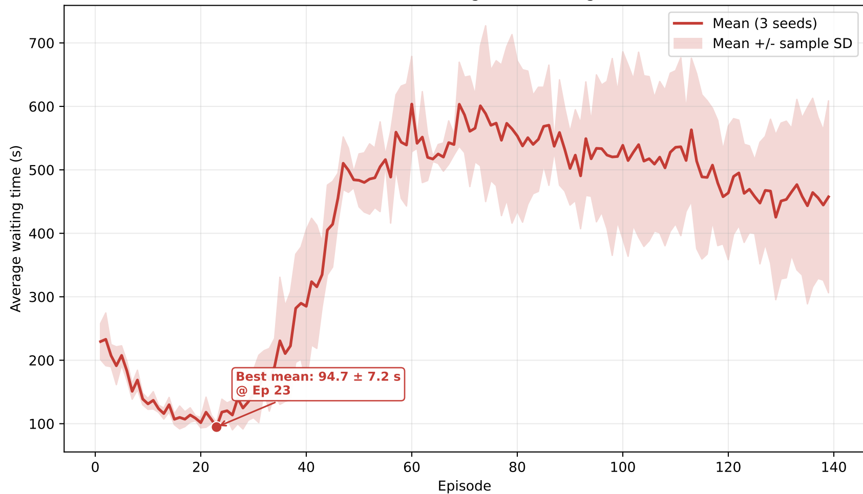
M05: three-seed waiting-time learning curve
