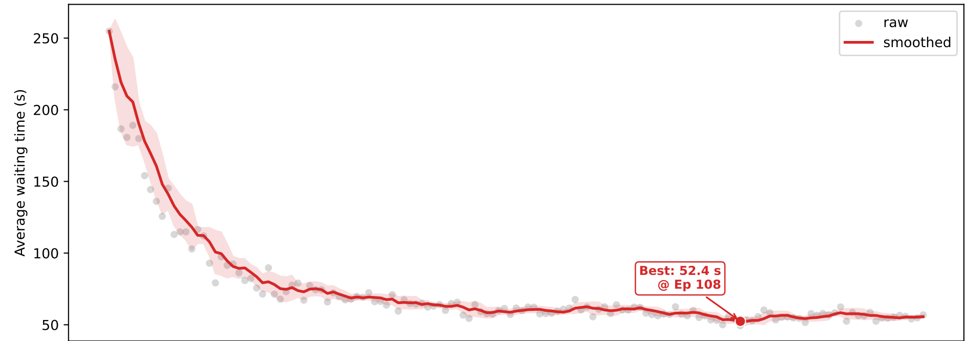
MARL queue fixed LR waiting time, run 1
