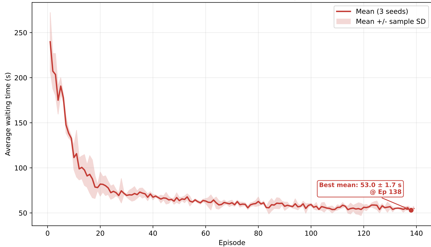
M01: three-seed waiting-time learning curve
