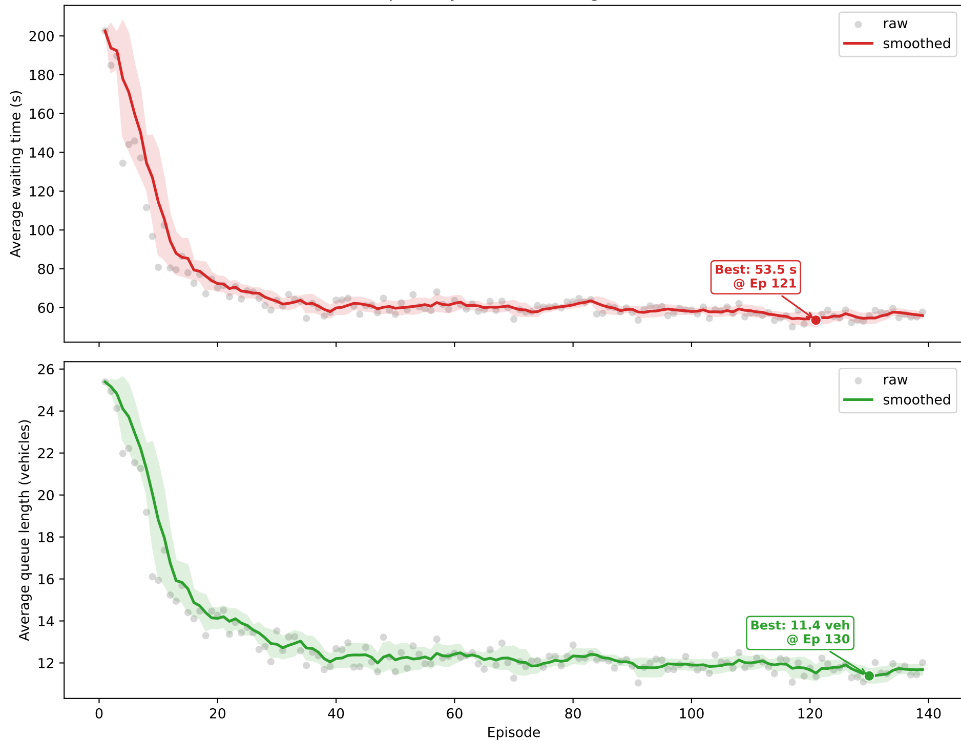
MARL queue dynamic LR waiting time, run 2
