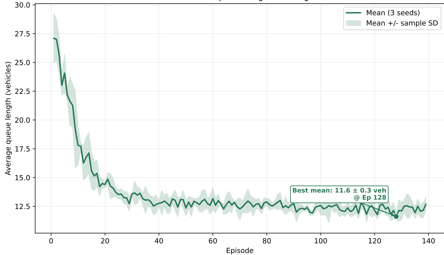
M02: three-seed queue-length learning curve
