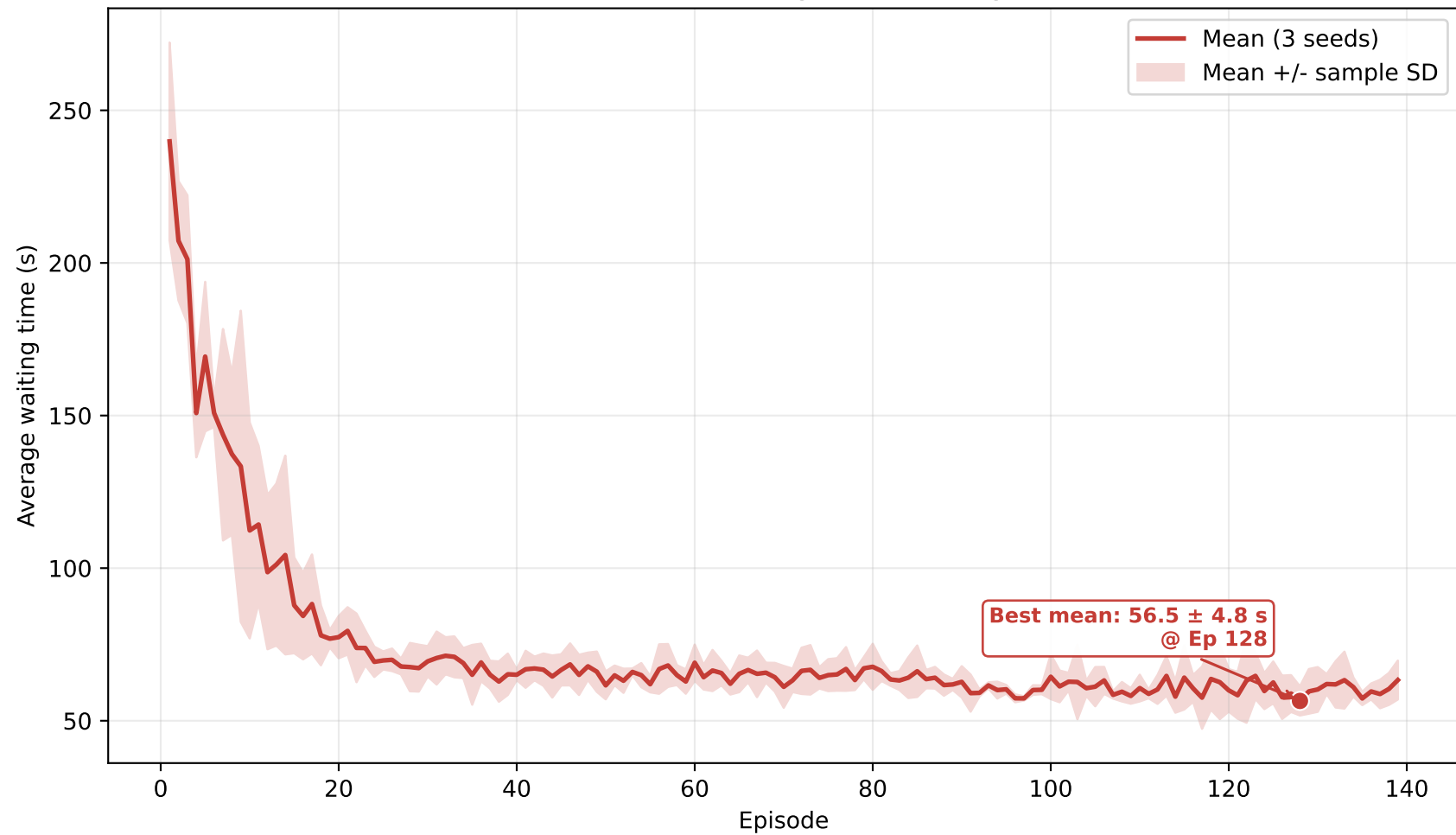
M02: three-seed waiting-time learning curve
