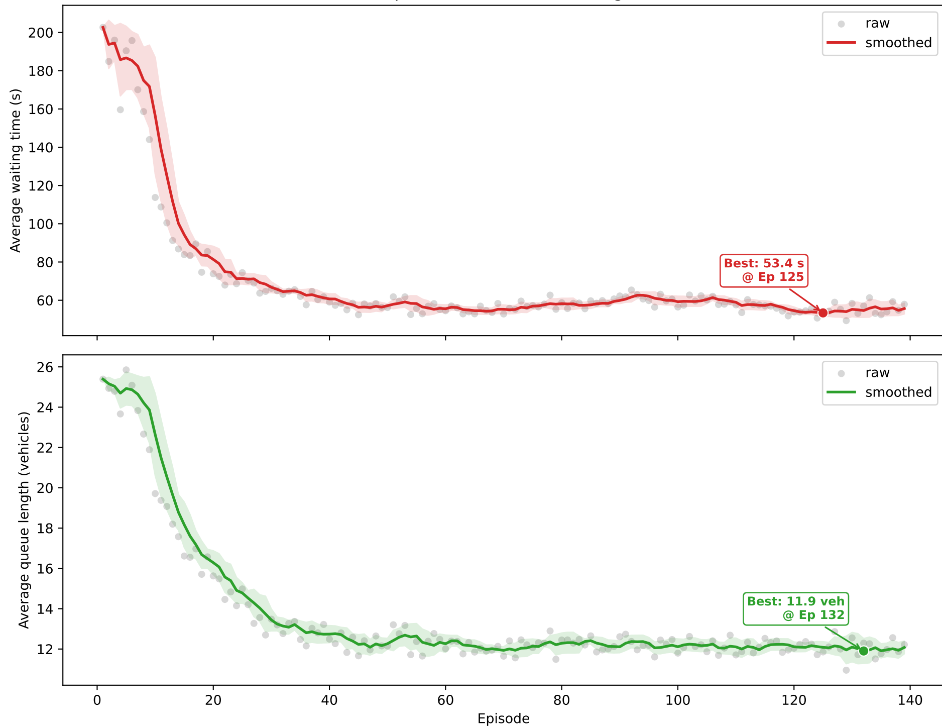
MARL active-phase PBRS fixed LR waiting time, run 2
