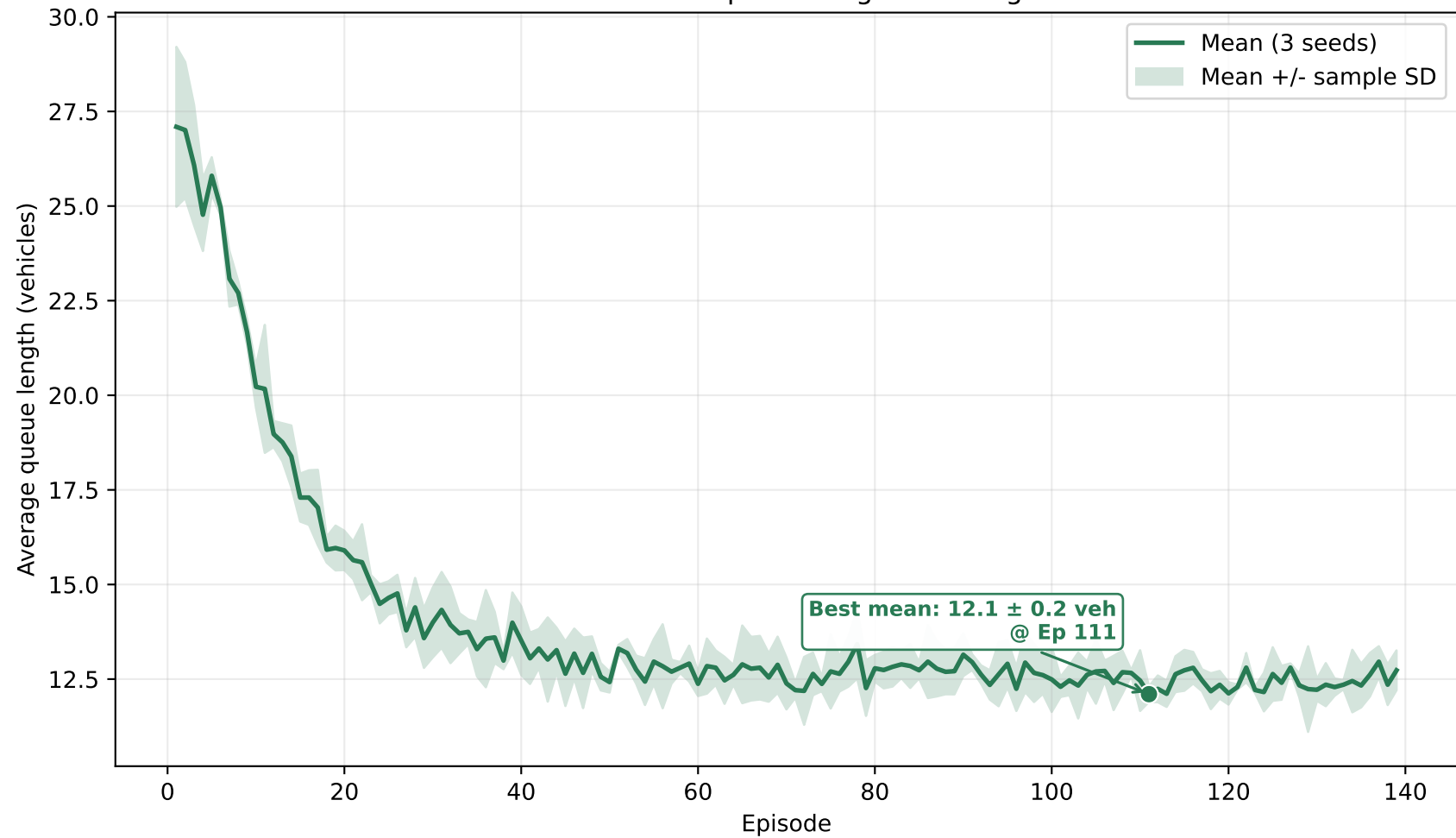
M03A: three-seed queue-length learning curve
