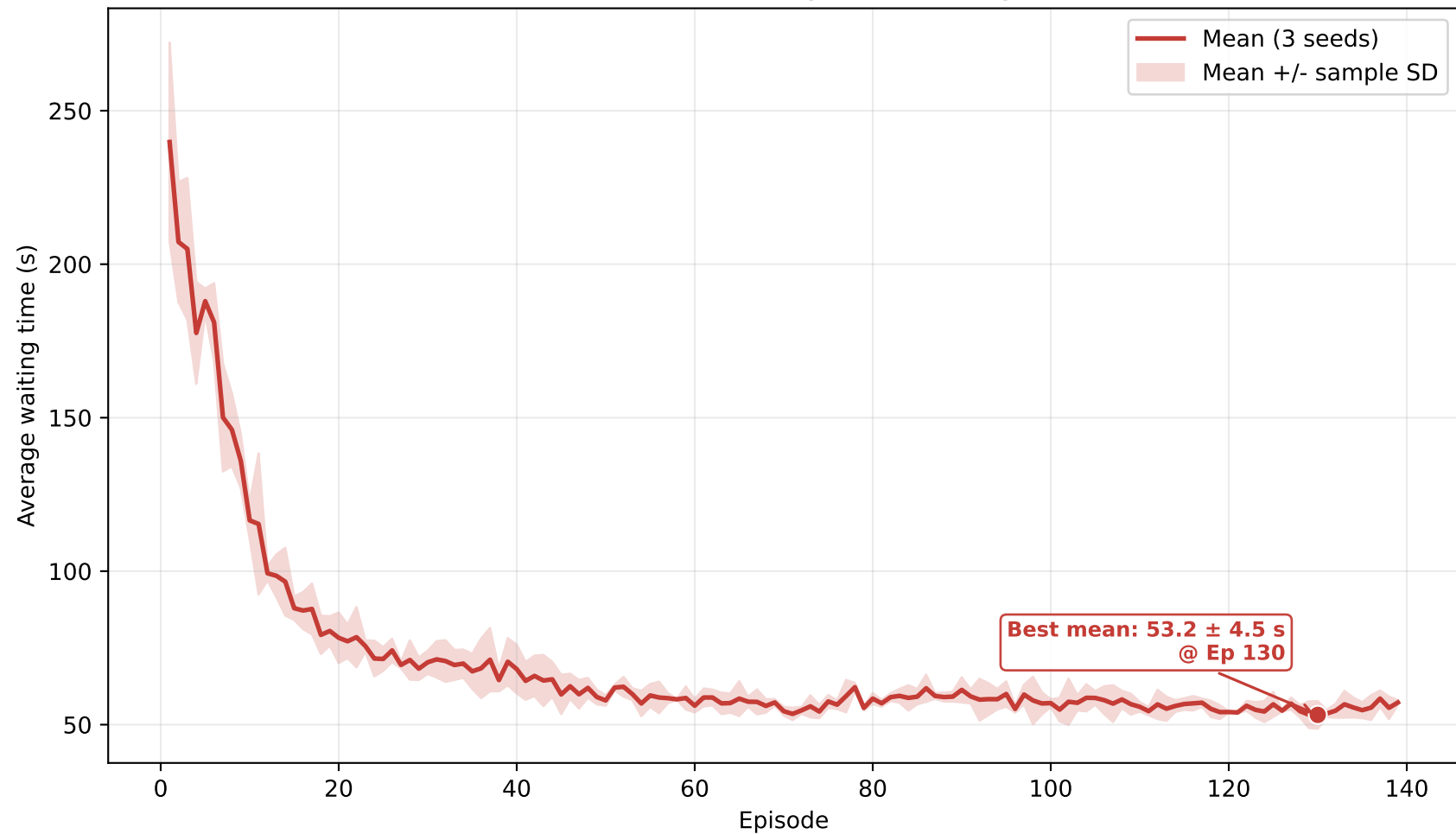
M03A: three-seed waiting-time learning curve
