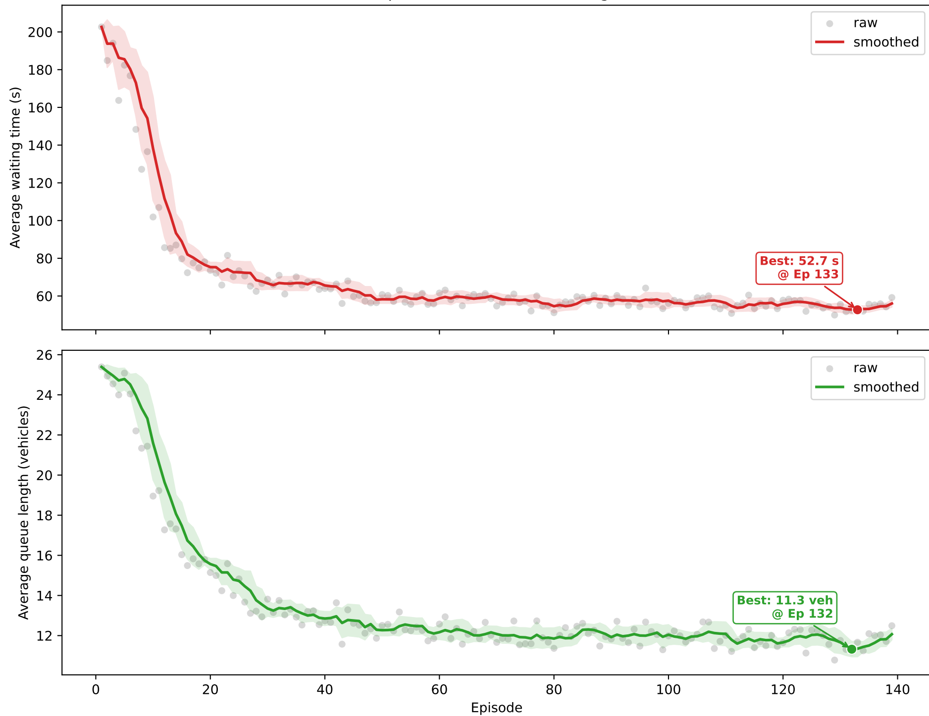
MARL total-queue PBRS fixed LR waiting time, run 2
