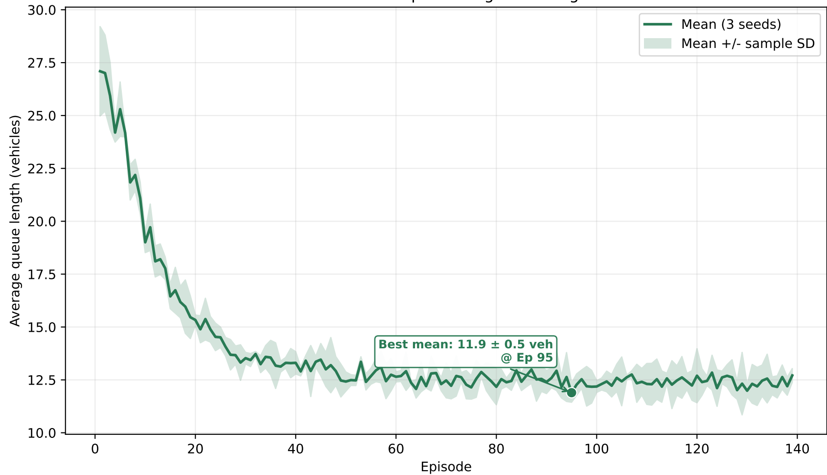
M03T: three-seed queue-length learning curve
