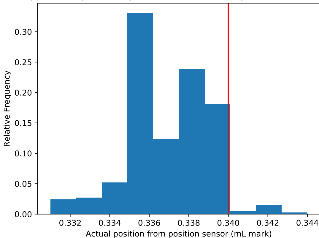
Pipettor PID positioning distribution with a target of 0.34 mL mark
