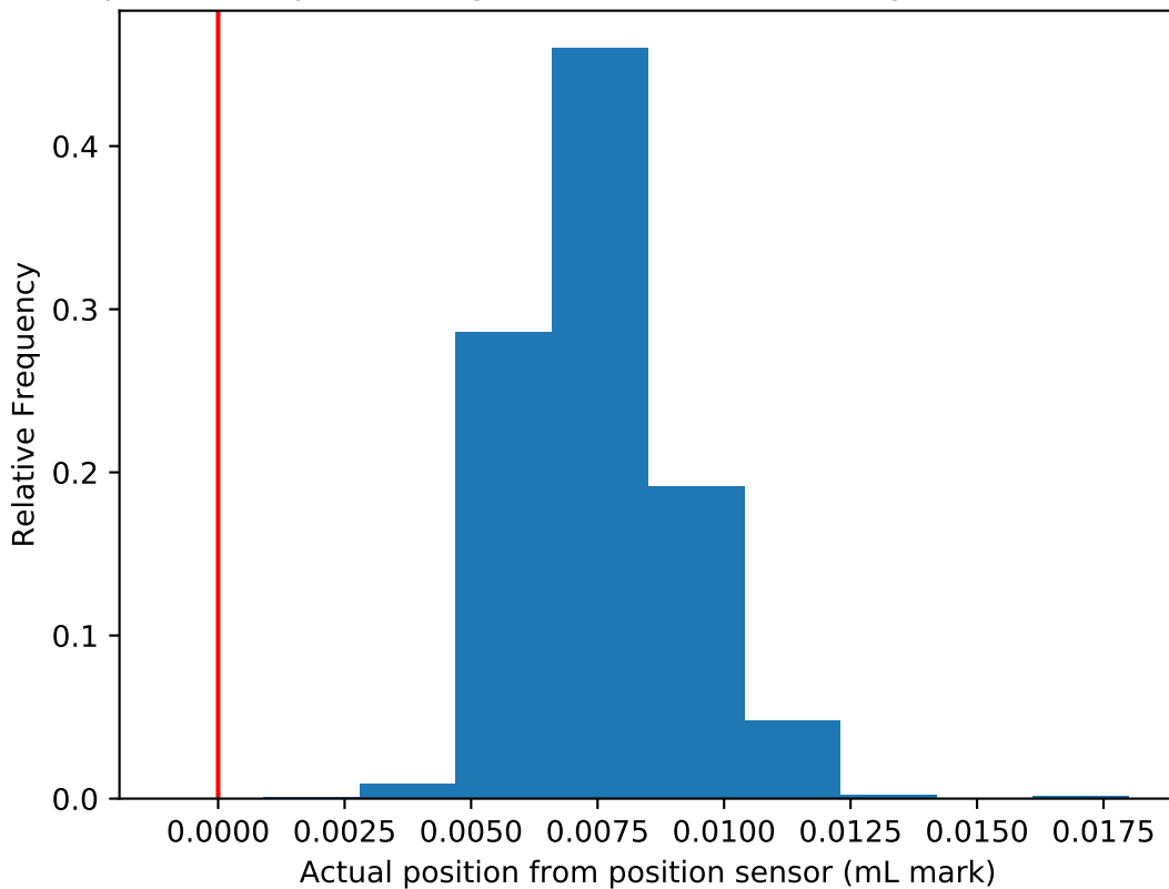
Pipettor PID positioning distribution with a target of 0.0 mL mark
