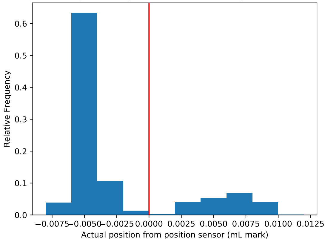
Pipettor PID positioning distribution with a target of 0.0 mL mark
