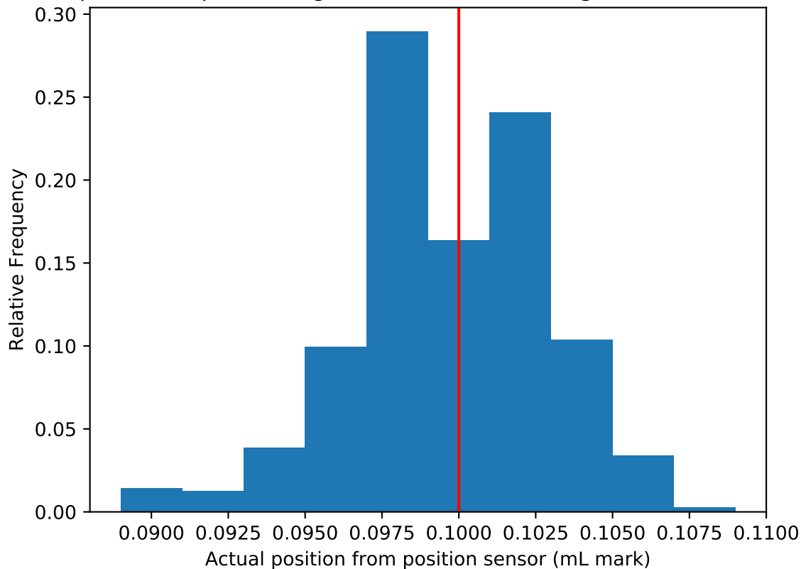
Pipettor PID positioning distribution with a target of 0.1 mL mark
