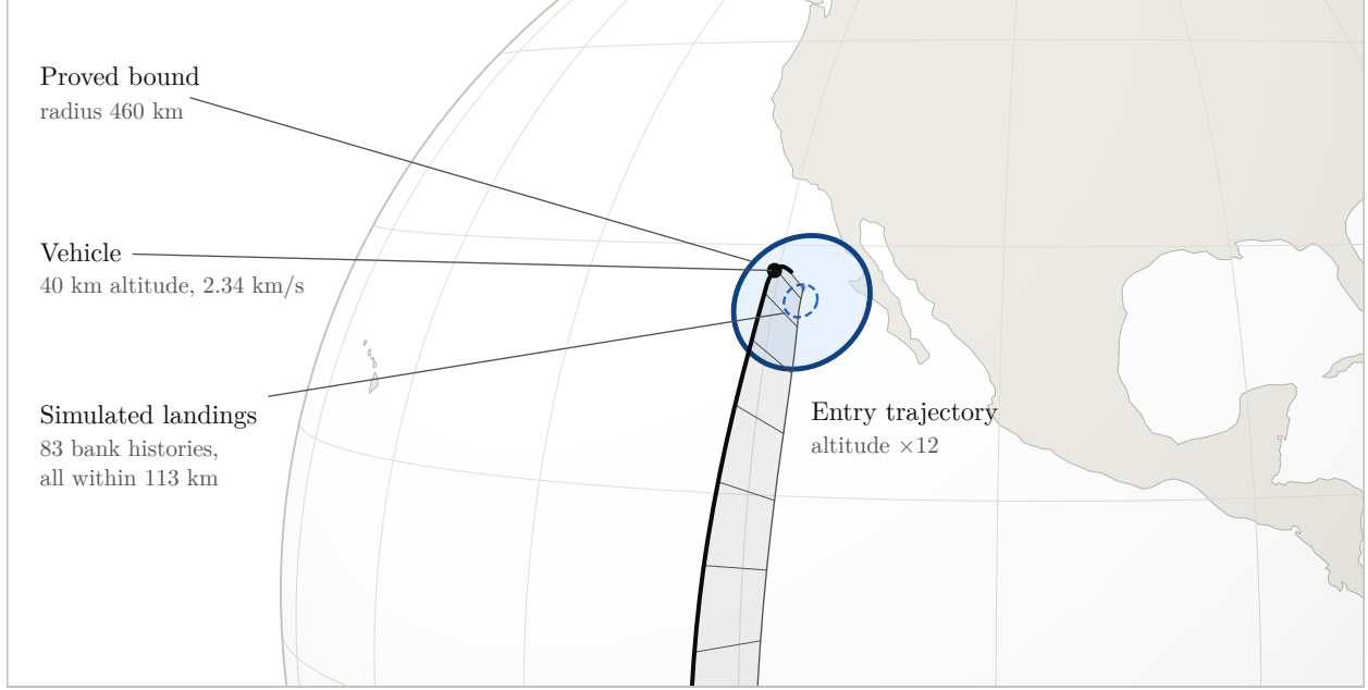
Figure 2.3: The bound of Proposition 2.1, evaluated on the example. The view is that of Fig. 2.2, enlarged about the end of the entry, so that the entry interface is out of the frame; the trajectory is the same simulated skip entry, with altitude drawn twelve times too large and a post marking each minute. From the state marked Vehicle , at which the vehicle last descends through 40 km, every bank history that keeps it below that altitude lands inside the solid circle. The landing points of a sweep of simulated bank histories from the same state lie inside the dashed circle. The solid circle is proved, and the dashed one is a sample.
