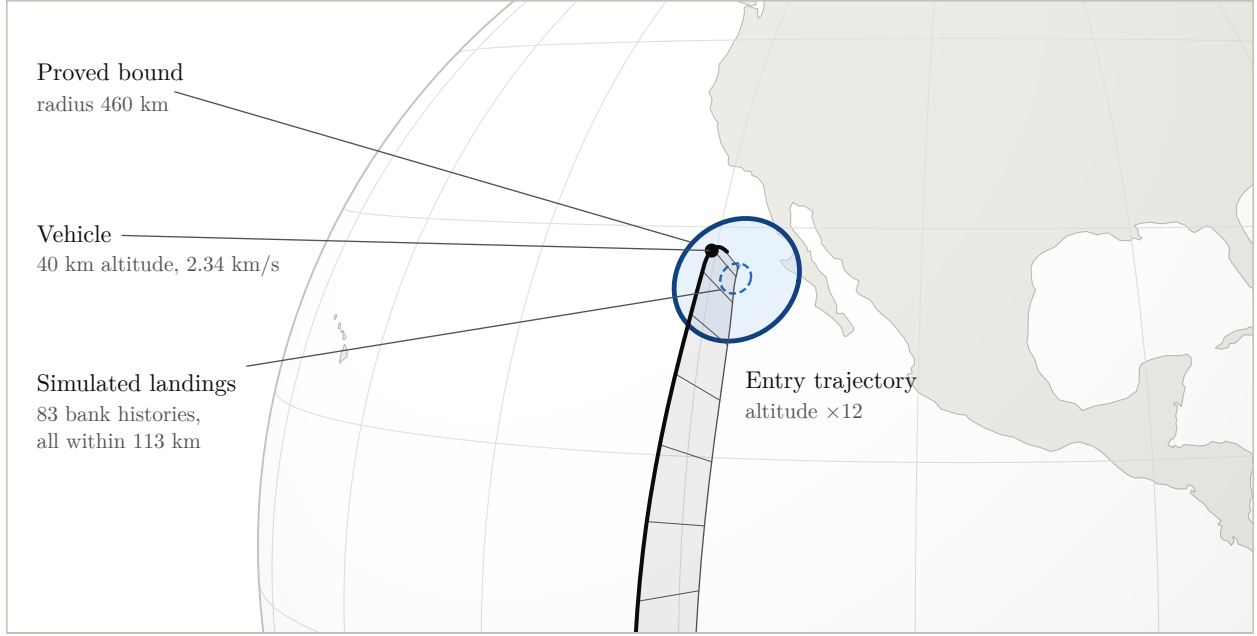
Figure 2.3: The bound of Proposition 2.1, evaluated on the example. The view is that of Fig. 2.2, enlarged about the end of the entry; the trajectory is the same simulated skip entry, with altitude drawn twelve times too large and a post marking each minute. From the state at which the vehicle last descends through 40 km, every bank history that keeps it below that altitude lands inside the solid circle. The landing points of a sweep of simulated bank histories from the same state lie inside the dashed circle. The solid circle is proved, and the dashed one is a sample.
