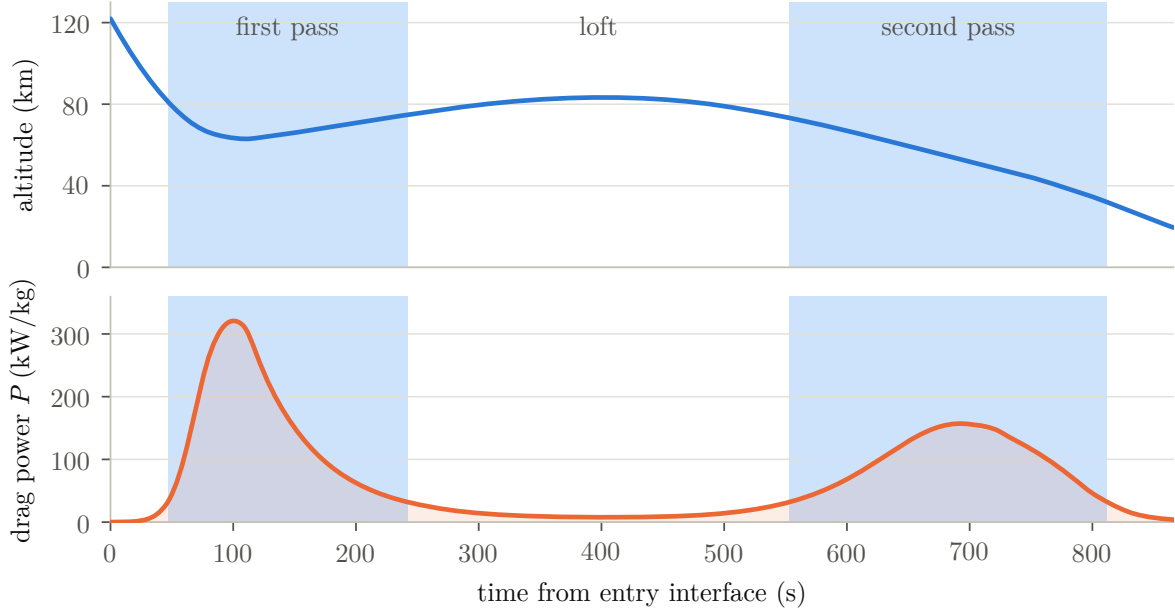
Figure 2.1: A skip entry at the physical scale height. The example is the lunar return of Artemis I, simulated from the published entry state [21]. Top: altitude. Bottom: the drag power per unit mass P , which is the rate at which mechanical energy is dissipated. The shaded intervals are the two atmospheric passes, on which P exceeds one tenth of its peak; between them the vehicle lofts and dissipates little. An occupation measure weighs every interval by its length, whereas what distinguishes one trajectory from another is decided in the shaded intervals, which have no length in the limit.
