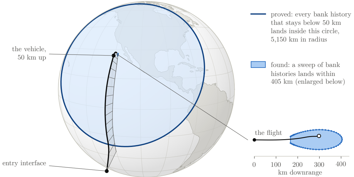
Figure 1: A first bound, on an example: a lunar-return skip entry simulated from a published entry state [2], with altitude drawn twelve times too large and a post marking each minute. The circle is proved, by the bound stated under A first bound ; the sweep is a sample of simulated bank histories from the same state. The program is to close the gap between the two.
