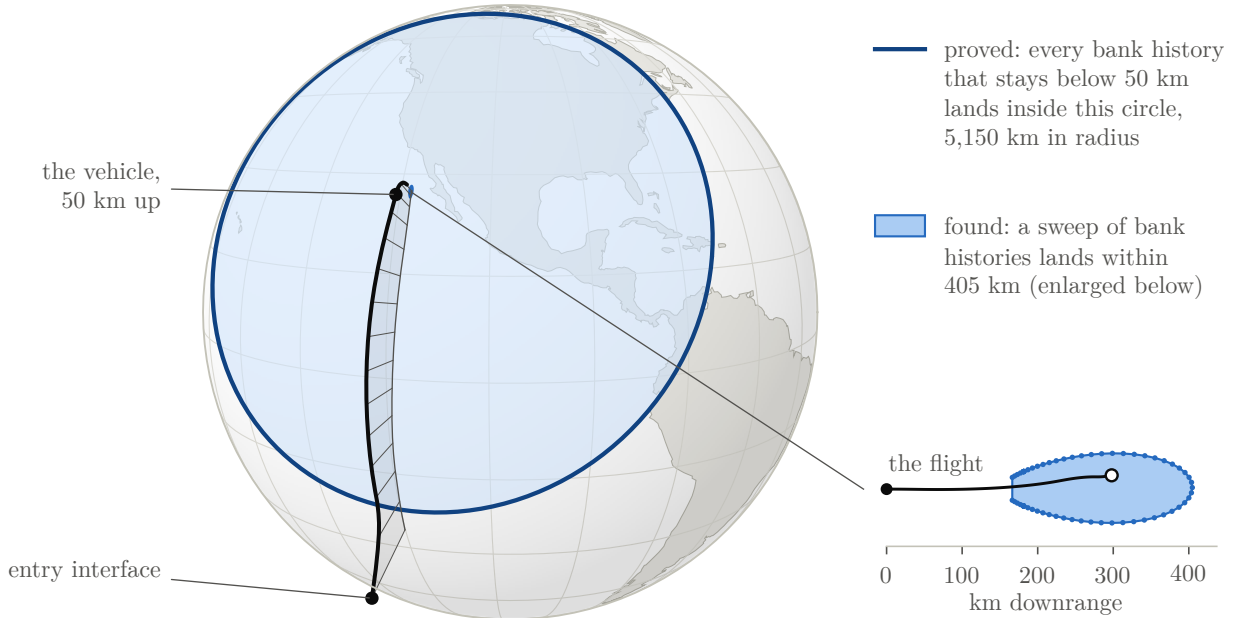
Figure 2.3: The bound of Proposition 2.1, evaluated on the example. The trajectory is the simulated skip entry of Fig. 2.2, with altitude drawn twelve times too large and a post marking each minute. From the point at which the vehicle last descends through 50 km, every bank history that keeps it below that altitude lands inside the circle. The landing points of a sweep of simulated bank histories from the same state are shown enlarged on the right; the simulated flight ends at the open circle. The circle is proved, and the sweep is a sample.
