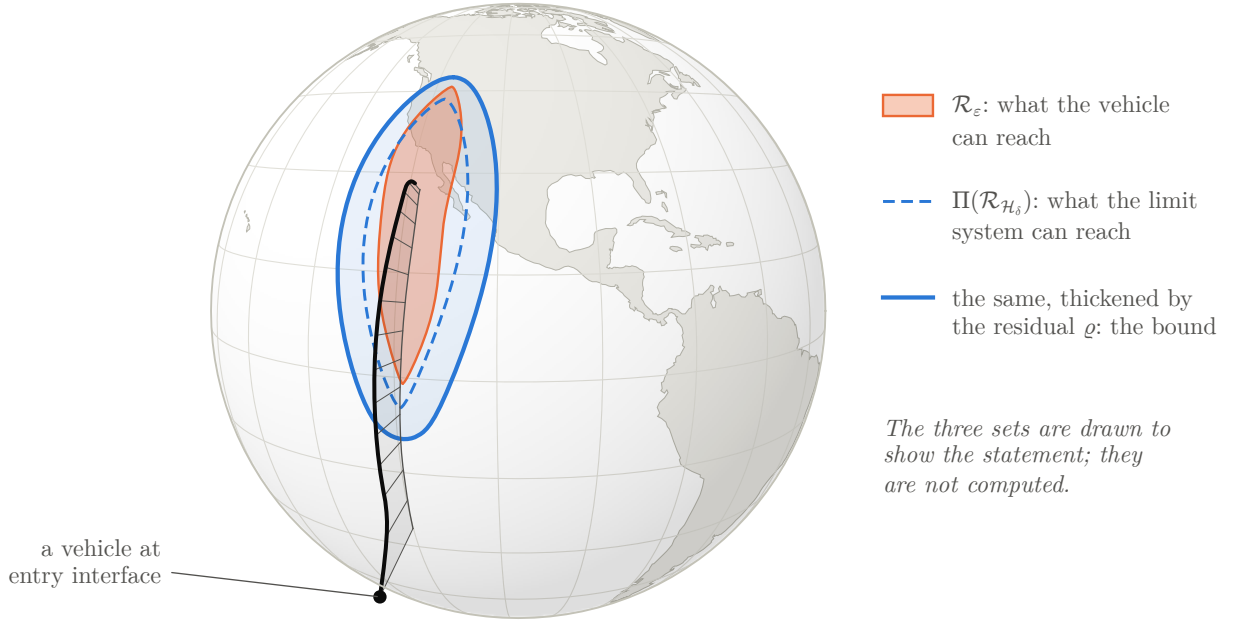
Figure 1: Illustration of the target statement, drawn on the ground. The trajectory is an example, a lunar-return skip entry simulated from a published entry state [2], with altitude drawn twelve times too large and a post marking each minute. The three sets are an illustration and are not computed: the set that the vehicle can reach, the set that the limit system can reach, and the latter thickened by the residual, which is the bound.
